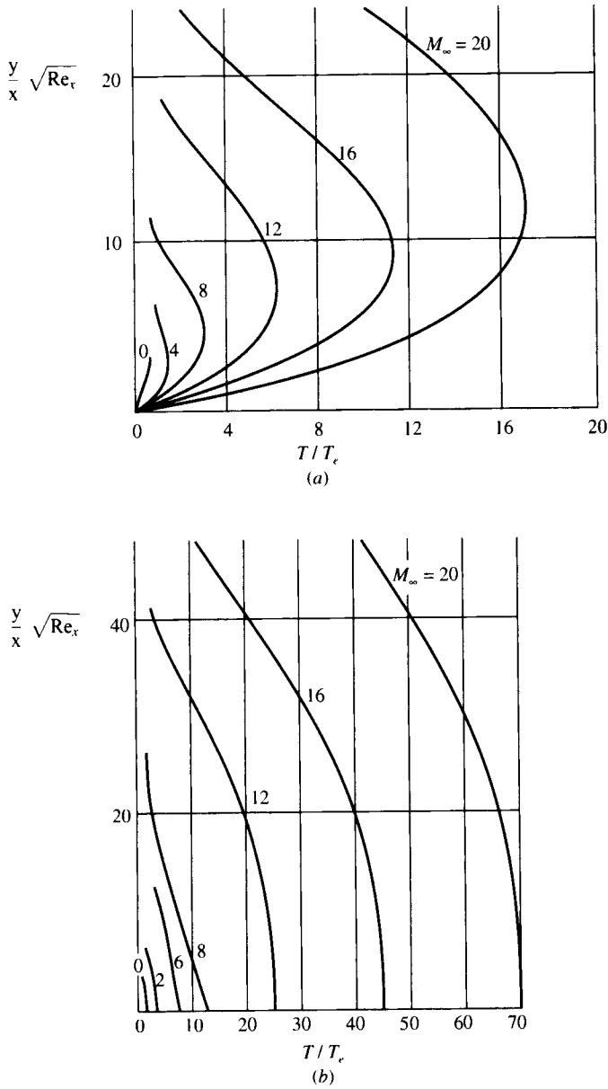
FIG. 10.13 Temperature profiles in a laminar compressible boundary layer. (a) Constant-temperature wall; (b) adiabatic wall. (Ref. 75.)
