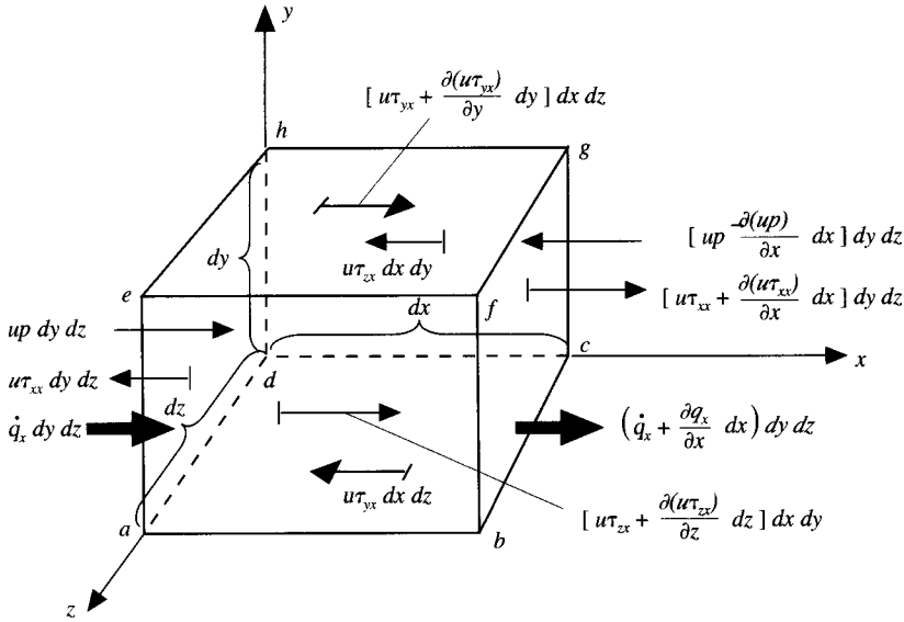
FIG. 2.10 Energy fluxes associated with an infinitesimally small, moving fluid element. For simplicity, only the fluxes in the x direction are shown. Model used for the derivation of the energy equation.
