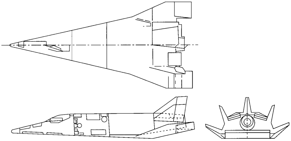
FIG. 12.1 Three-dimensional view of the X-24C hypersonic test vehicle.
