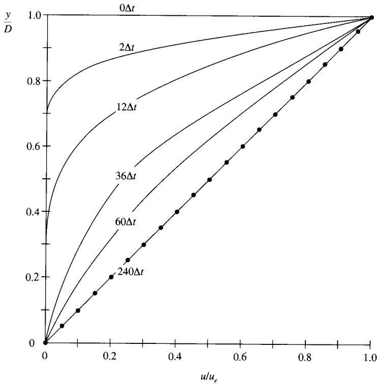
FIG. 9.4 Velocity profiles for unsteady Couette flow at various stages in the time-stepping process. Solid circles are exact analytical solution (steady state); solid lines are numerical solutions.
