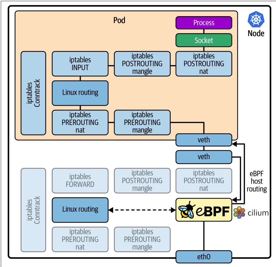
Figure 8-6. Bypassing iptables and conntrack processing with eBPF
