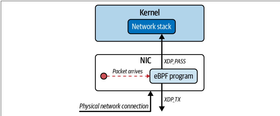
Figure 8-3. Network interface cards that support XDP offload can process, drop, and retransmit packets without any work required from the host CPU
