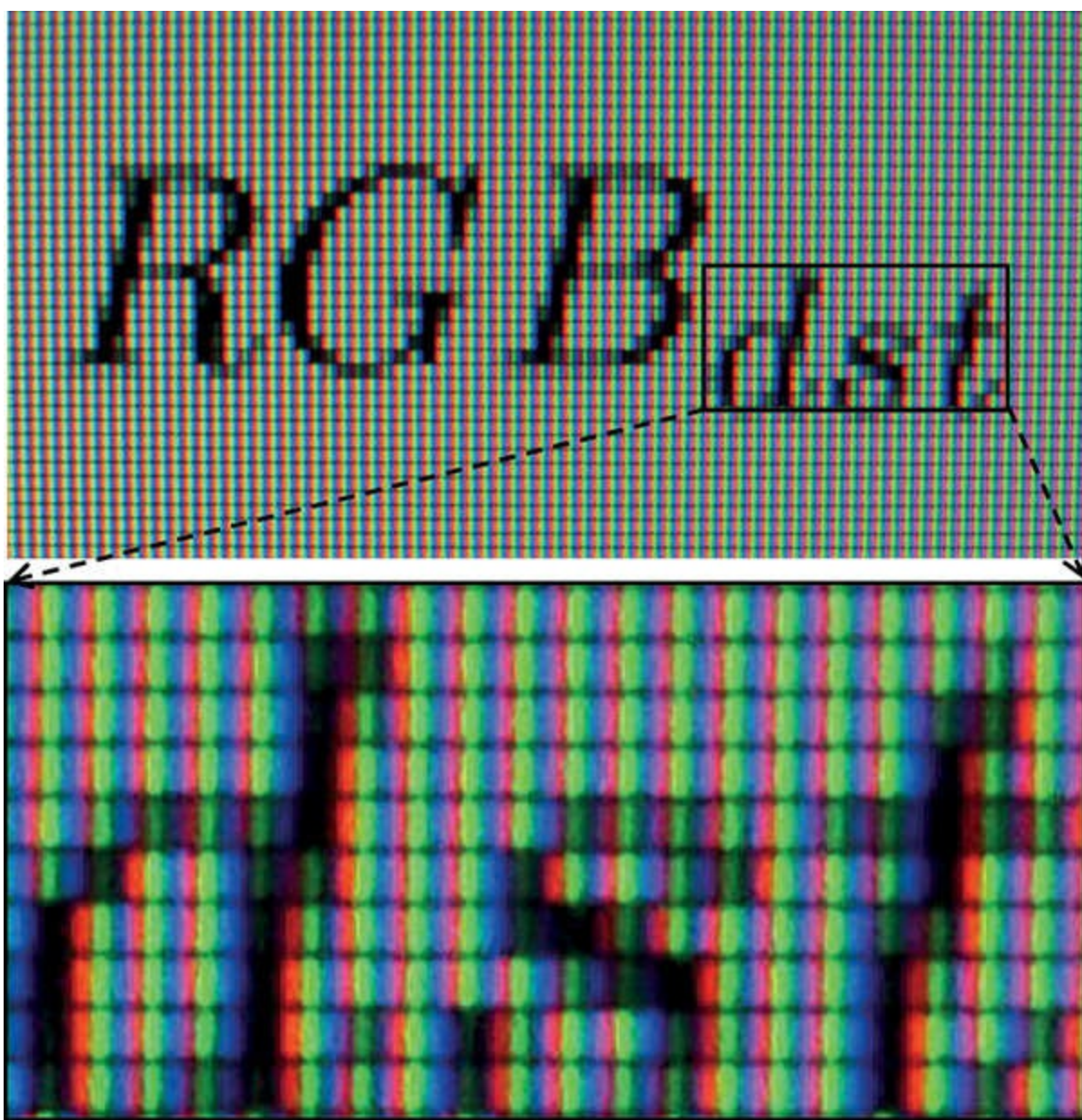
Figure 6.23 Close-up of RGB color elements in an LCD panel
