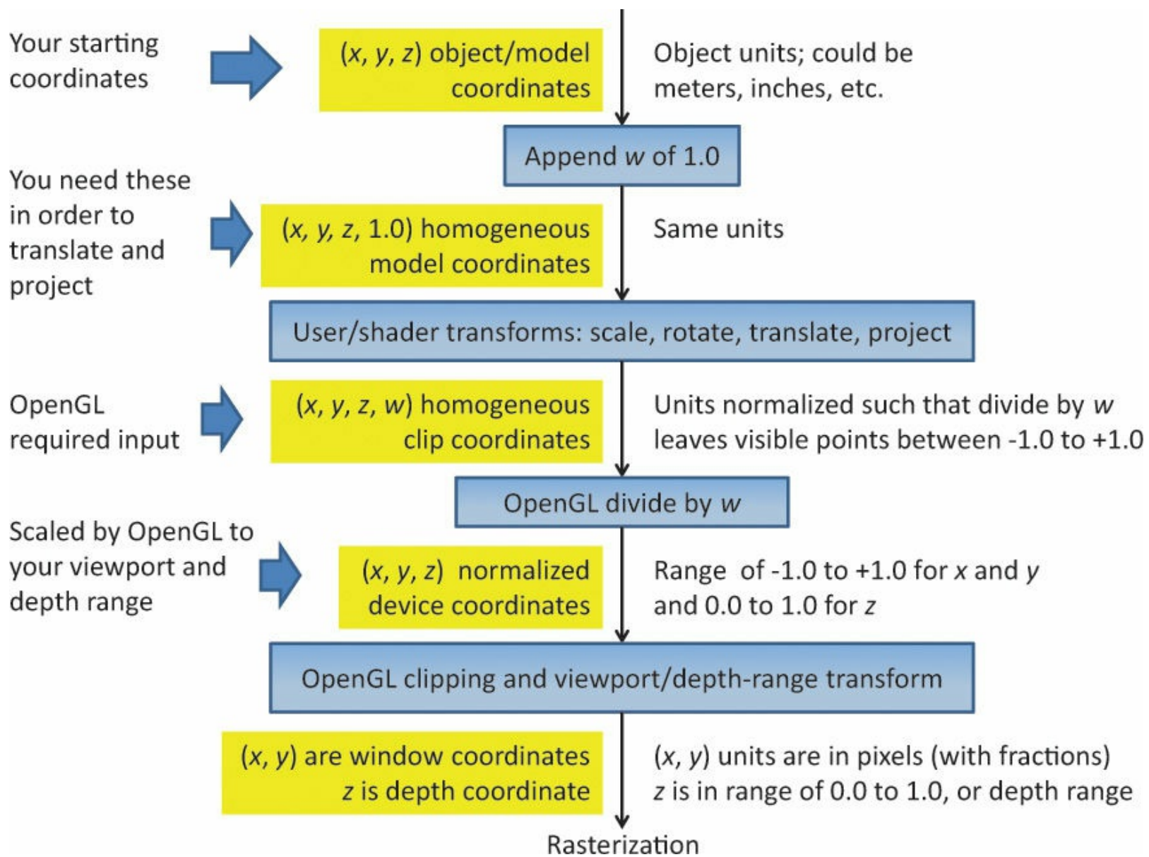
Figure 5.2 Coordinate systems required by OpenGL
