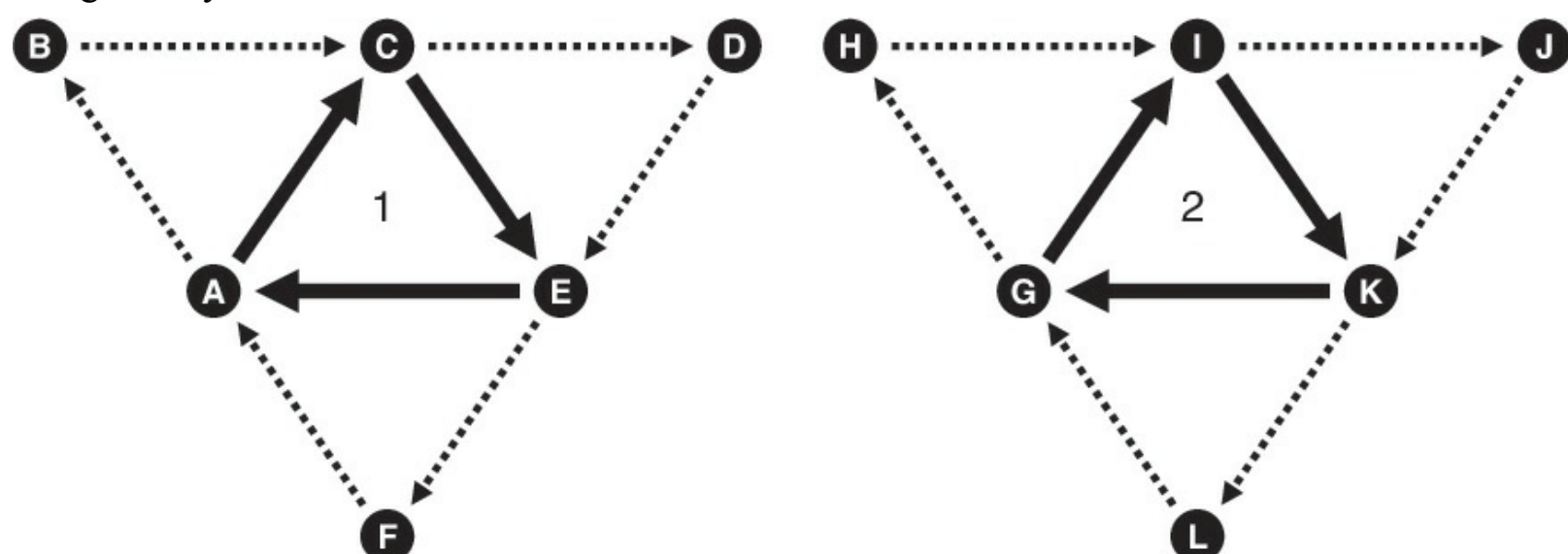
Figure 10.3 Triangles adjacency sequence Vertex sequence for GL_TRIANGLES_ADJACENCY primitives.
