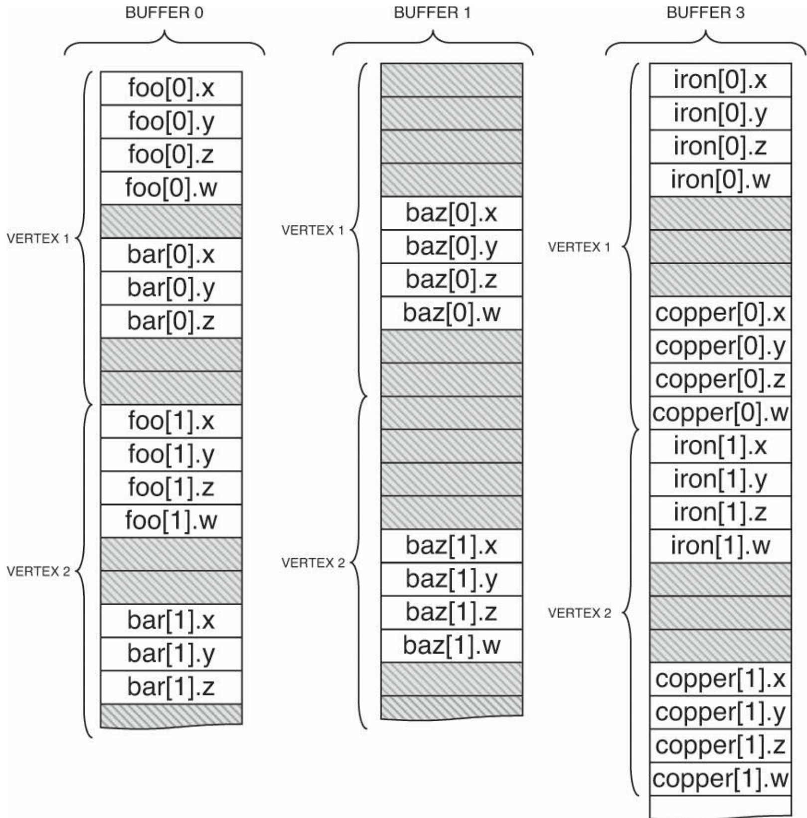
Figure 5.18 Transform feedback varyings packed into multiple buffers
