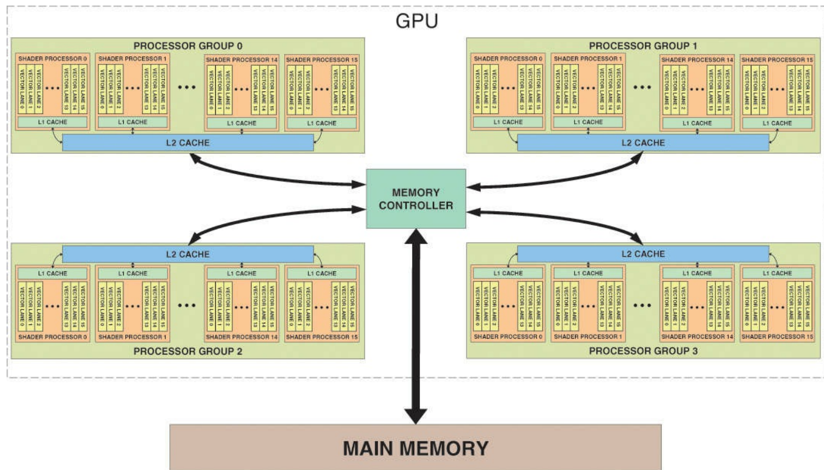
Figure 11.5 Cache hierarchy of a fictitious GPU
