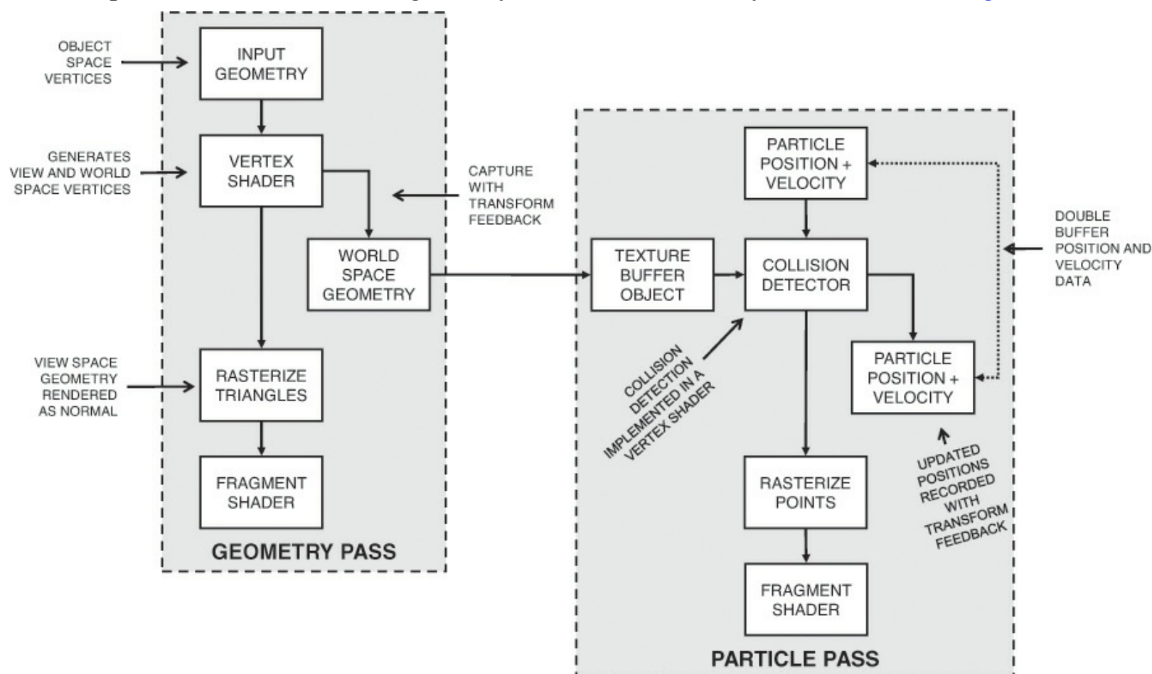
Figure 5.19 Schematic of the particle system simulator
