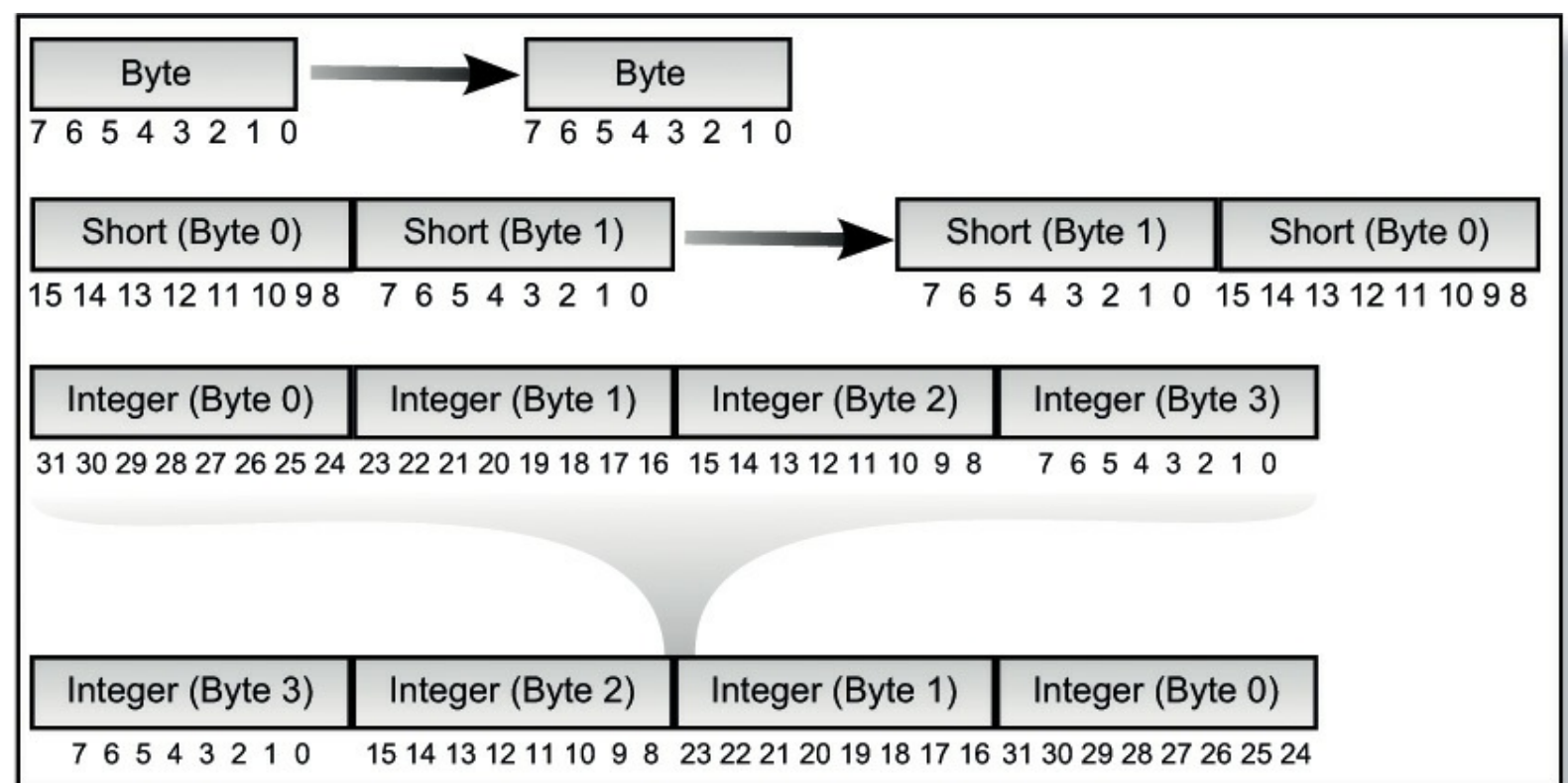
Figure 6.1 Byte-swap effect on byte, short, and integer data
