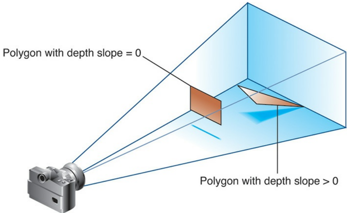
Figure 4.2 Polygons and their depth slopes
