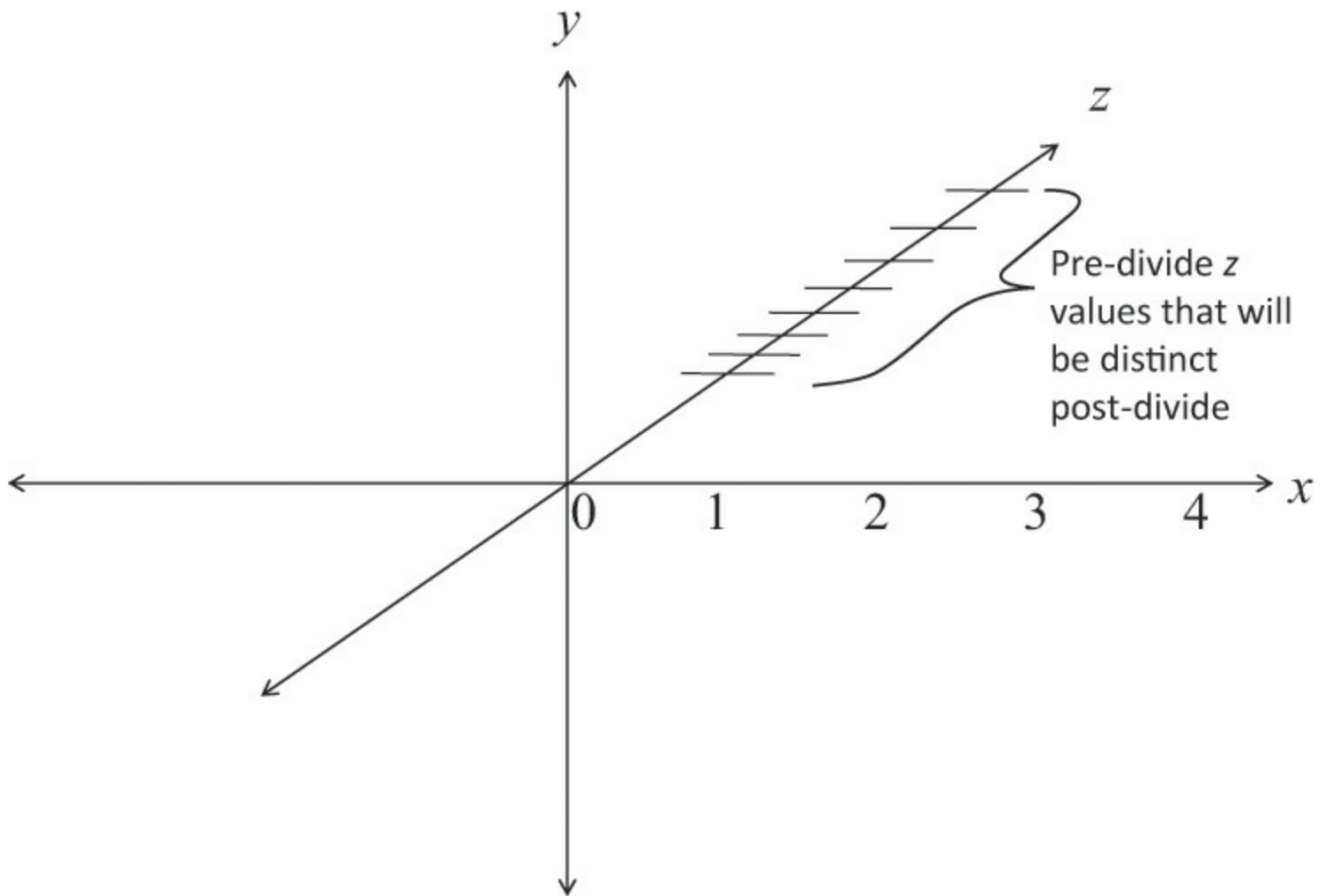
Figure 5.15 z precision
