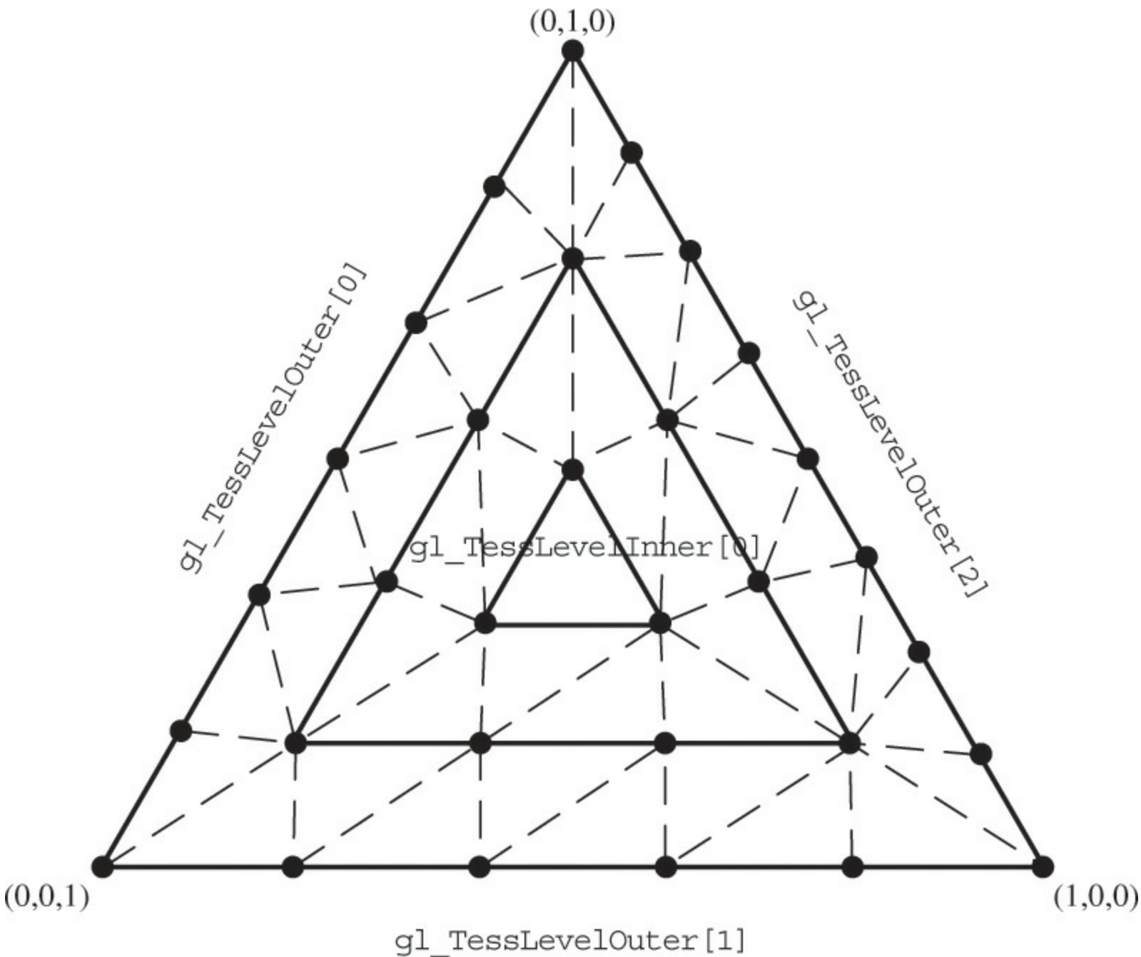
Figure 9.3 Triangle tessellation
