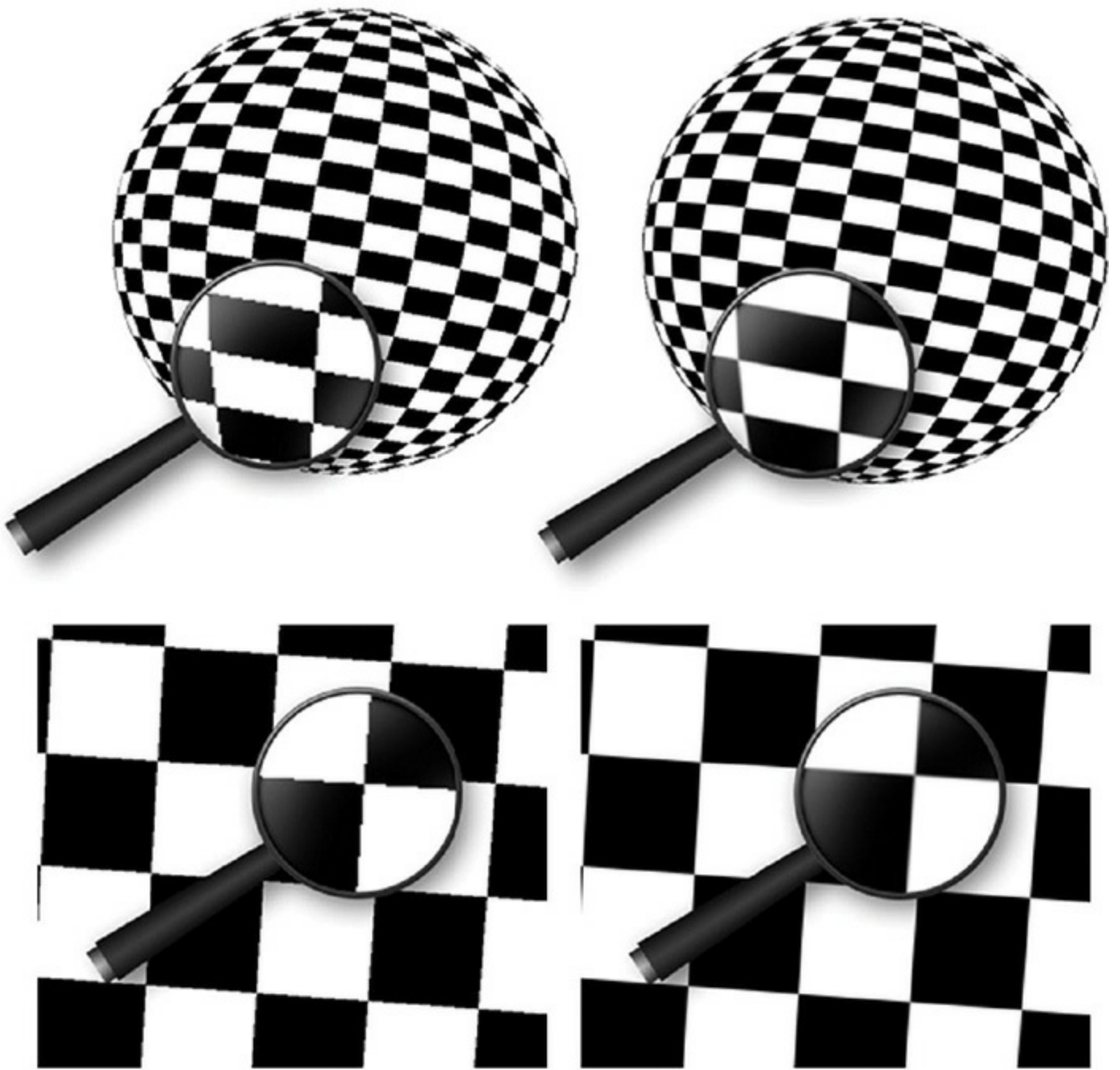
Figure 8.20 Checkerboard pattern
