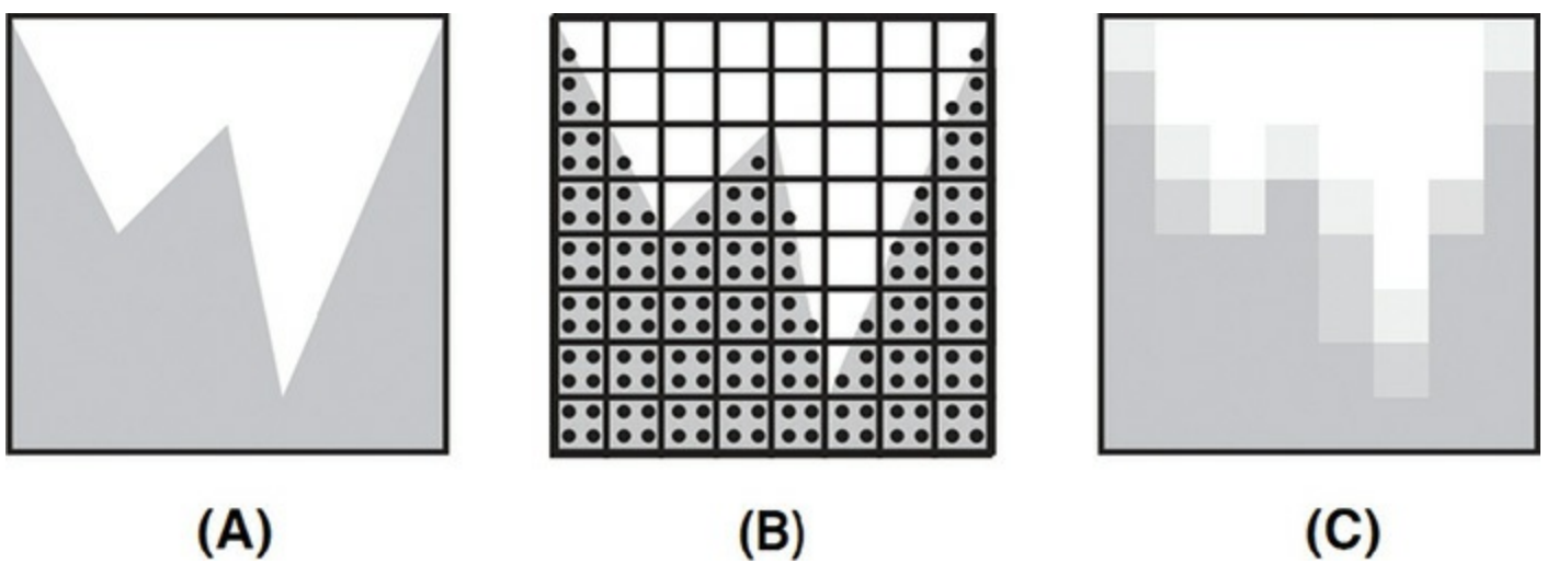
Figure 8.12 Supersampling
