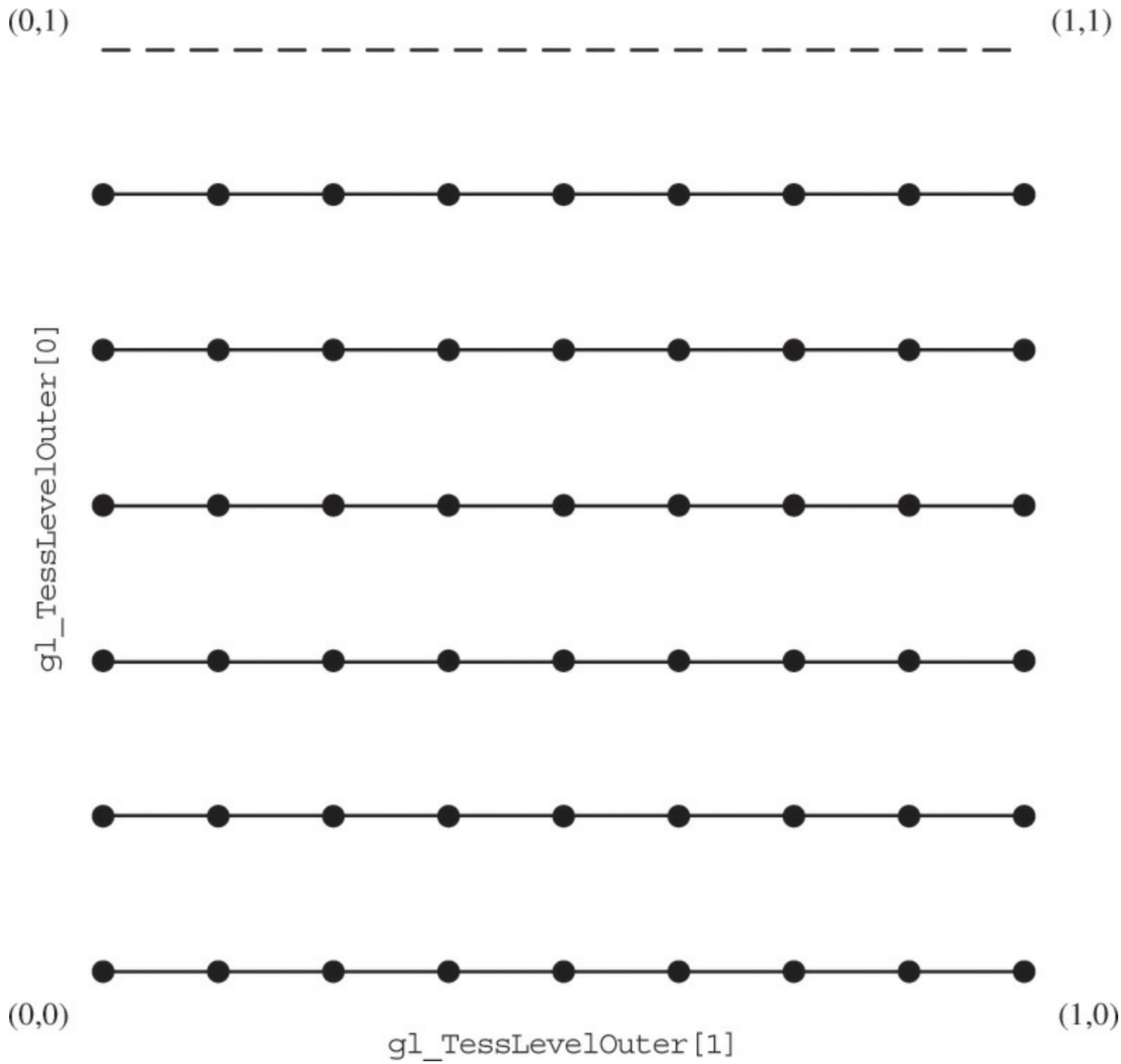
Figure 9.2 Isoline tessellation
