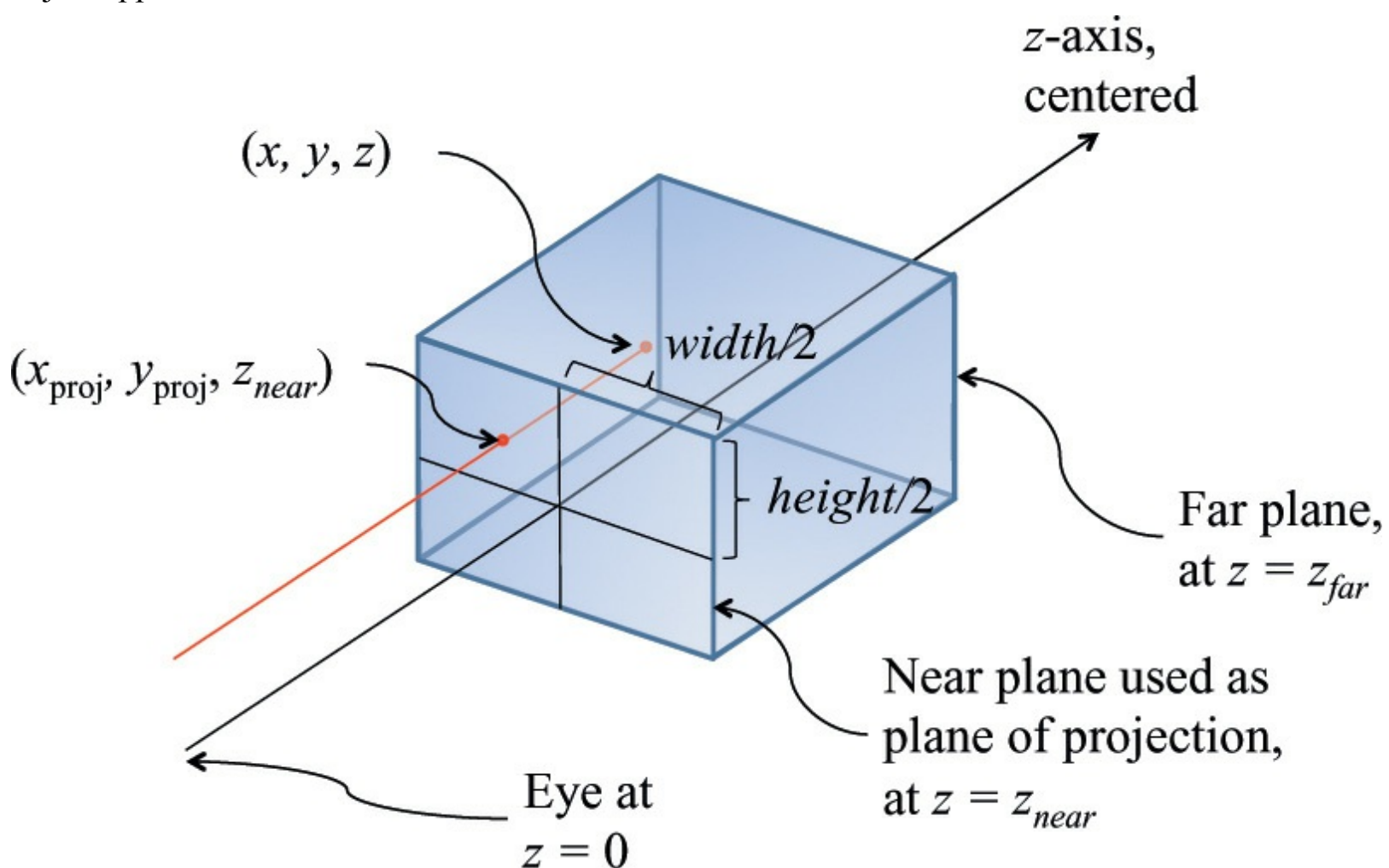
Figure 5.14 Orthographic projection
