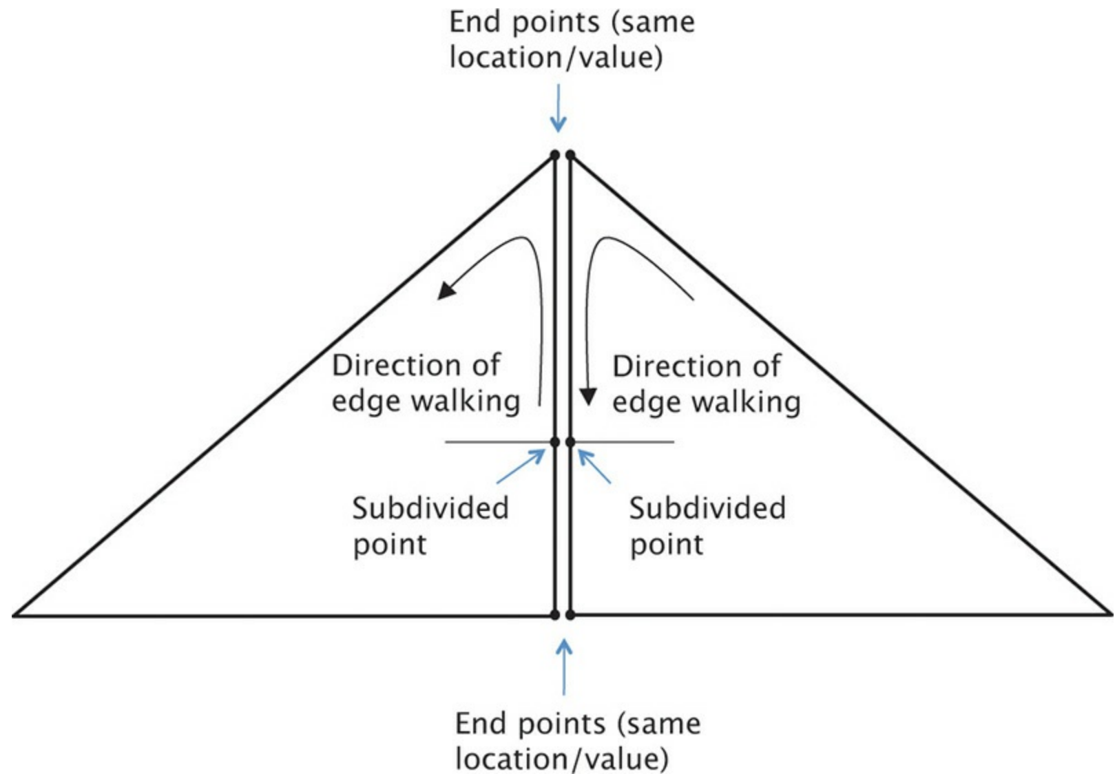
Figure 9.6 Tessellation cracking
