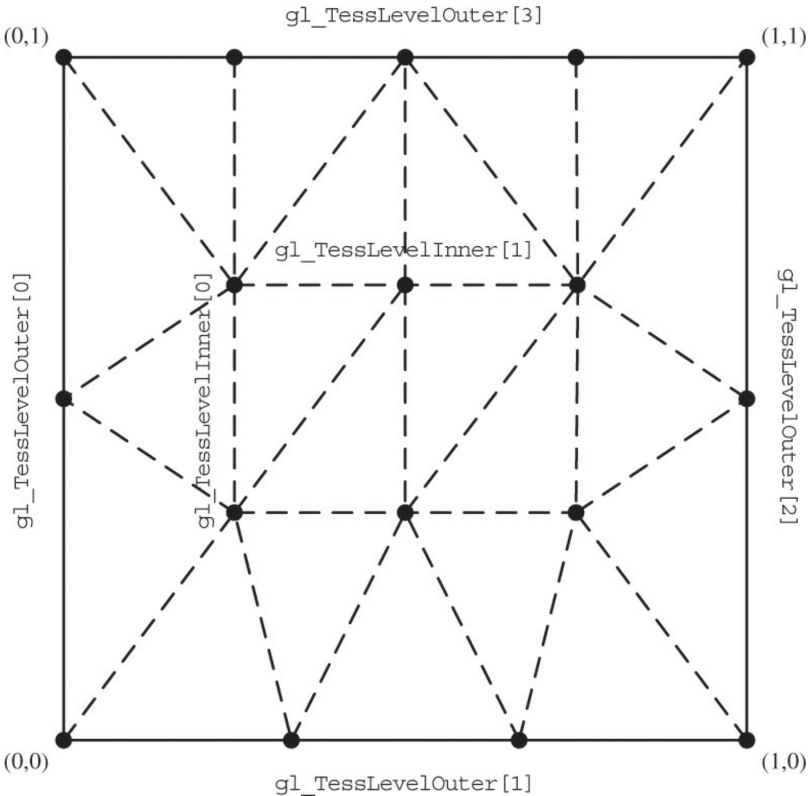
Figure 9.1 Quad tessellation
