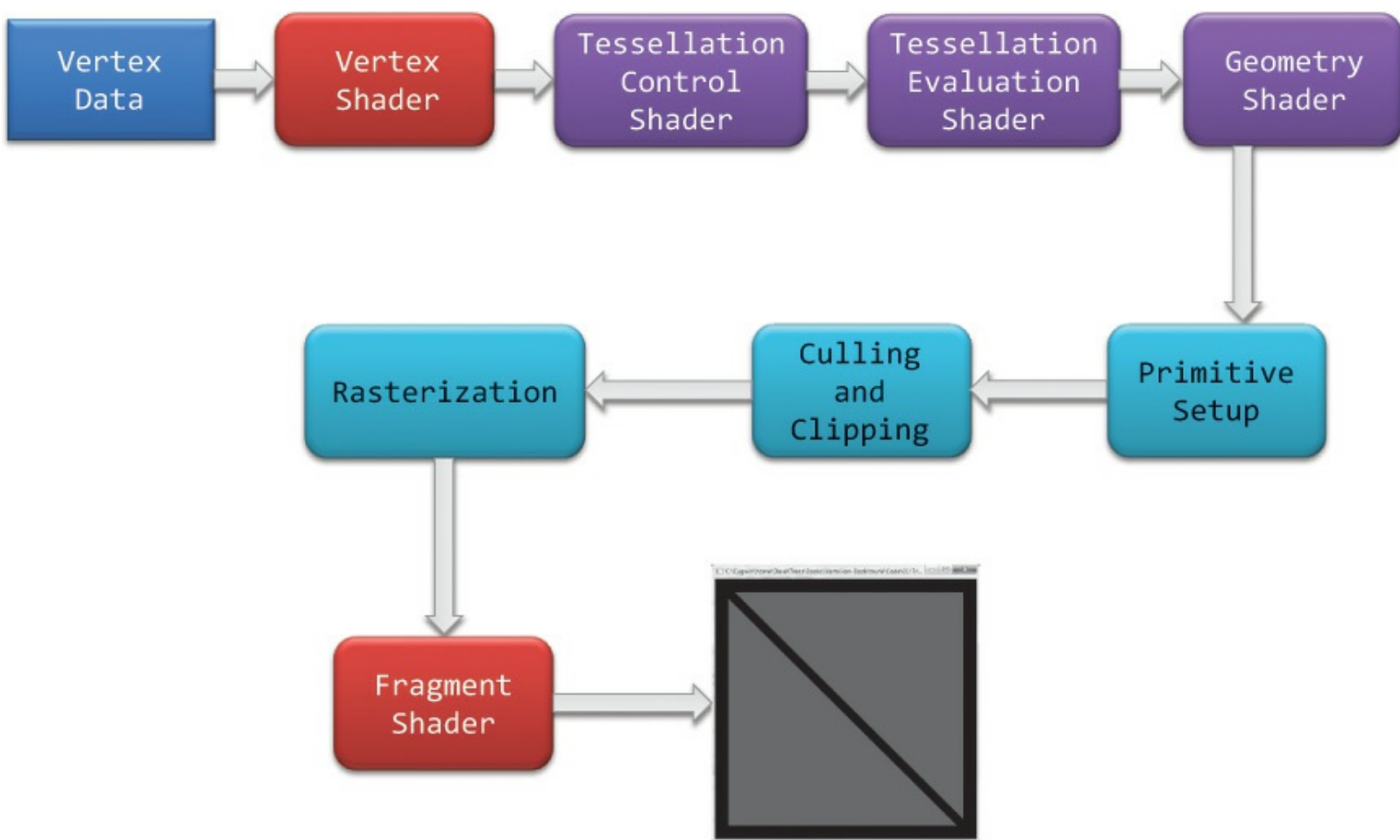
Figure 1.2 OpenGL pipeline
