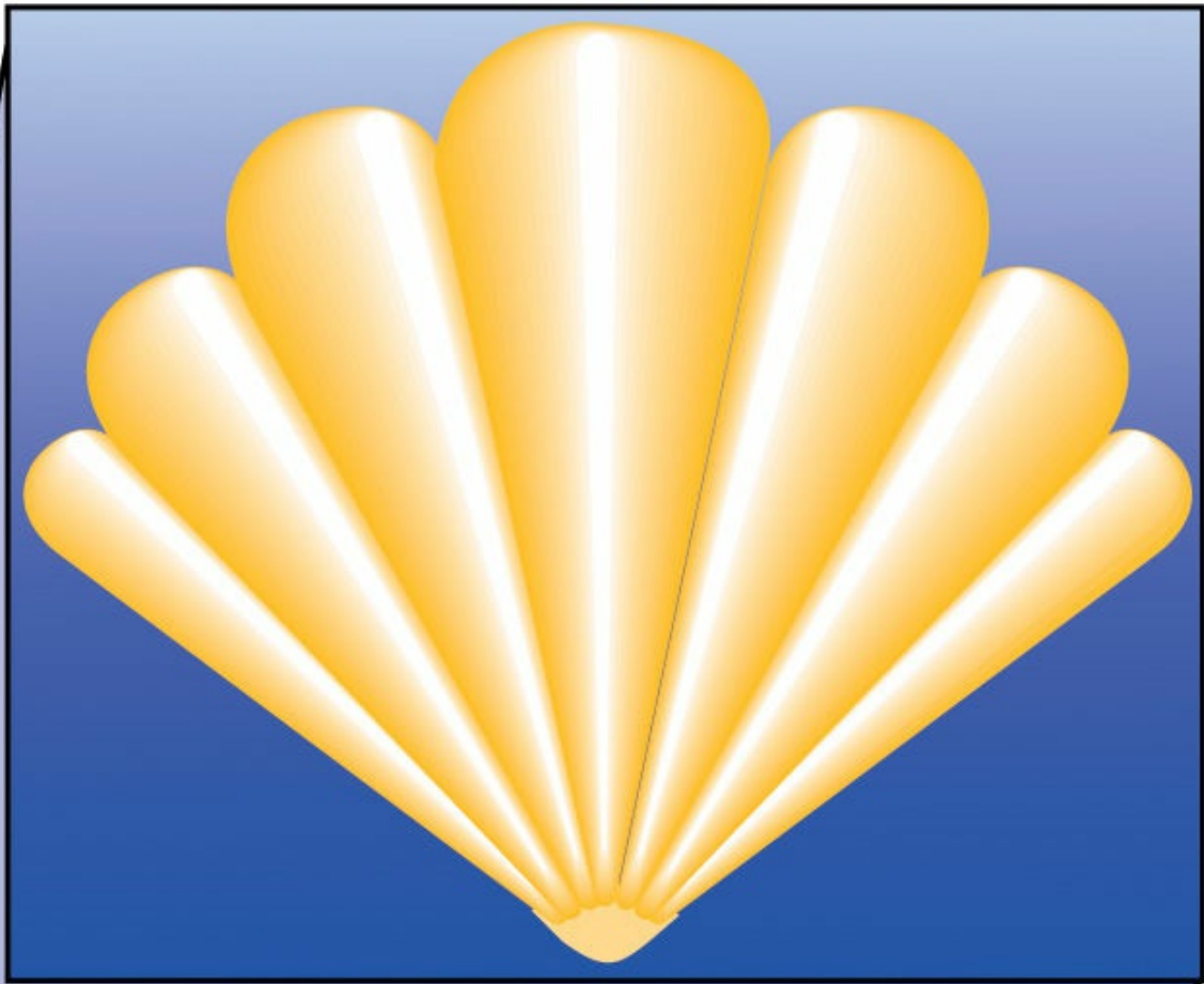
Original texture
