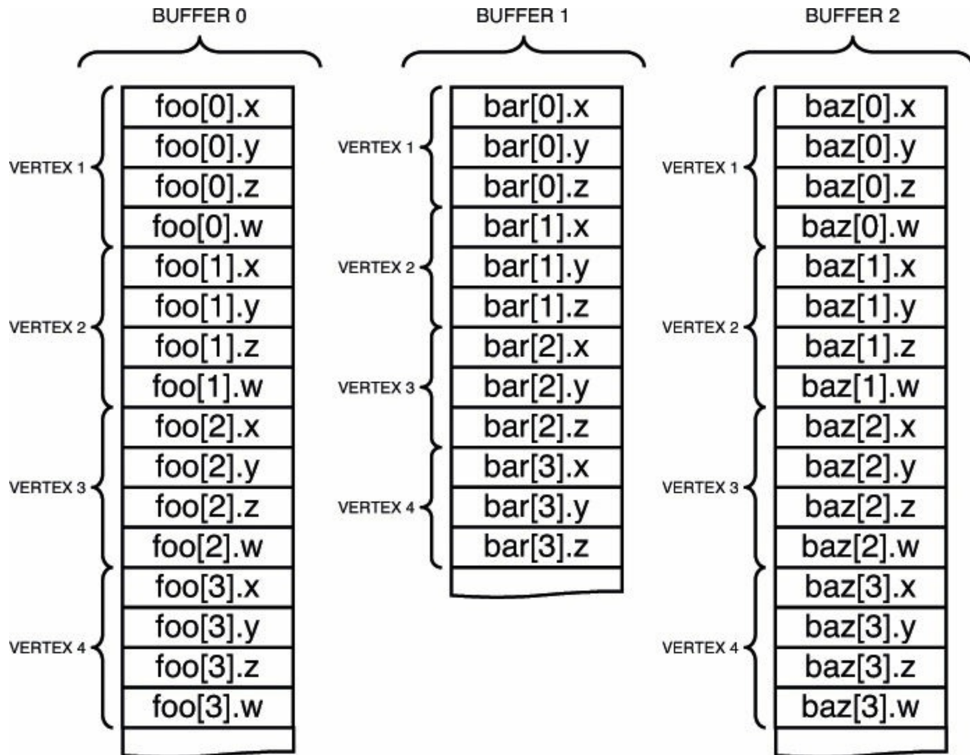
Figure 5.17 Transform feedback varyings packed in separate buffers
