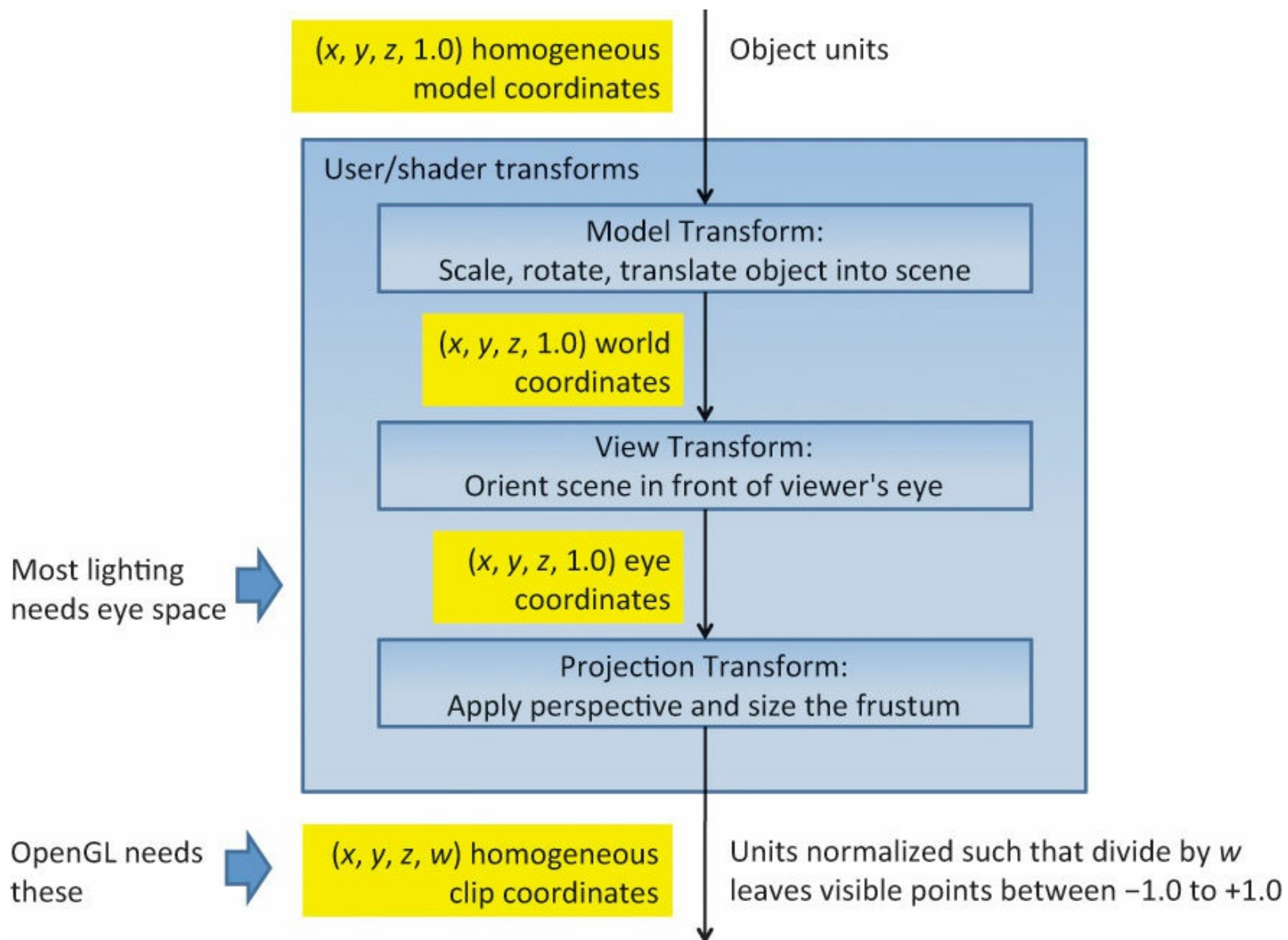
Figure 5.3 User coordinate systems unseen by OpenGL
