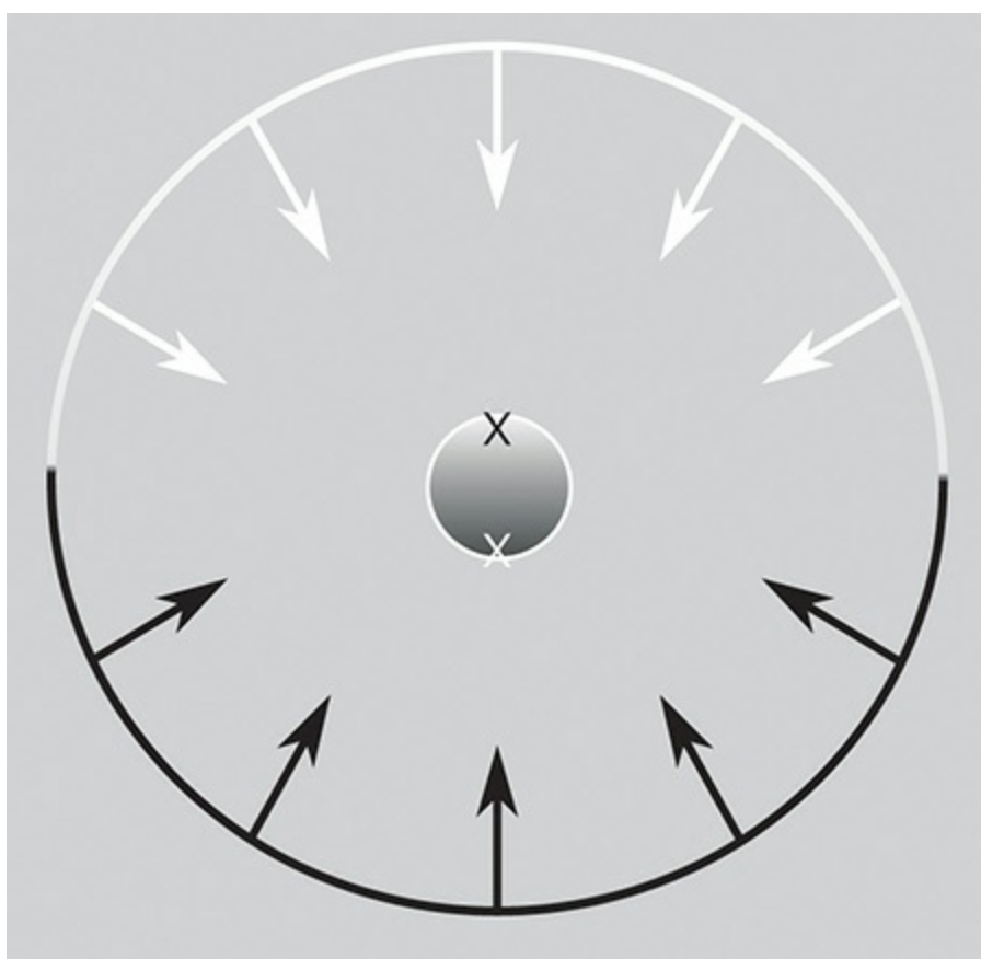
Figure 7.2 A sphere illuminated using the hemisphere lighting model
