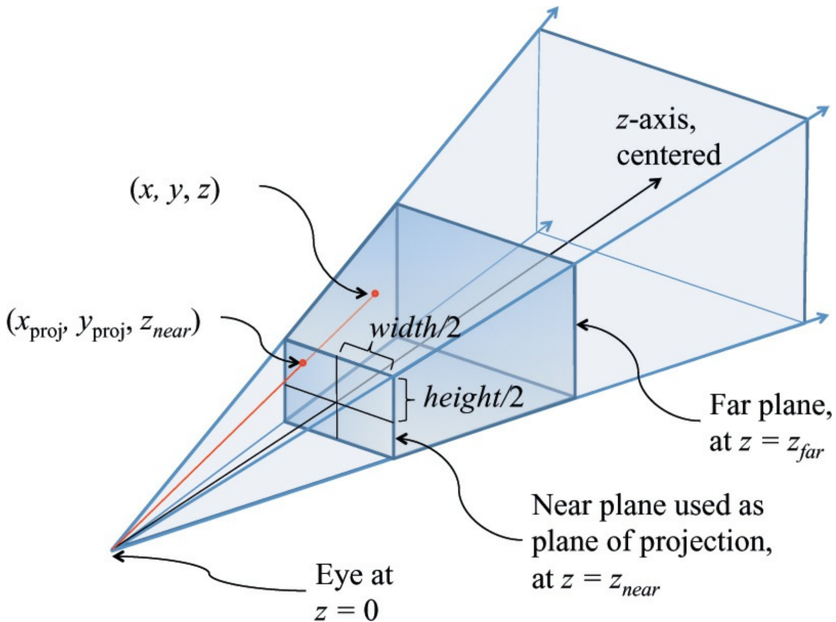
Figure 5.13 Frustum projection
