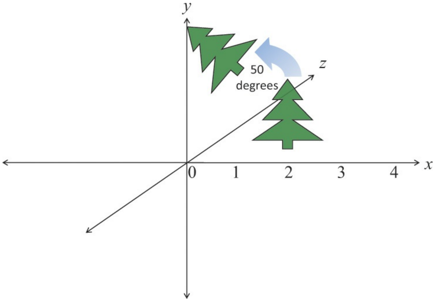
Figure 5.11 Rotation
