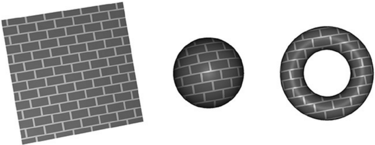
Figure 8.3 Brick patterns
