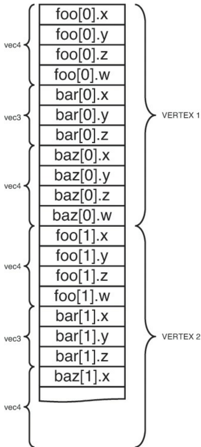
Figure 5.16 Transform feedback varyings packed in a single buffer
