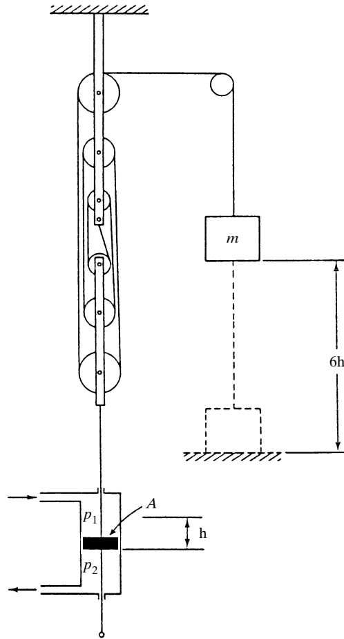
Figure 7-25 Six-pulley hoist.
