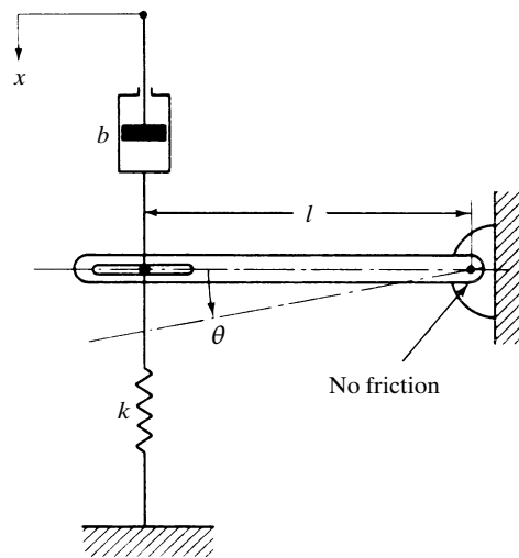
Figure 11-78 Mechanical system.
