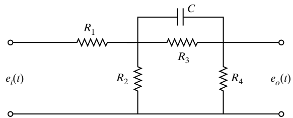
Figure 6-73 Electrical circuit.
