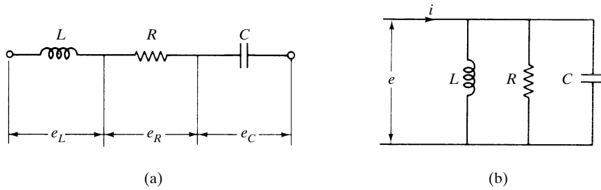
Figure 6-49 Electrical circuits.
