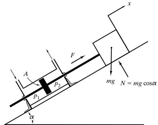
Figure 7-37 Pneumatic system.
