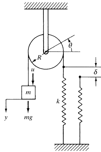
Figure 5-37 Spring-mass-pulley system.
