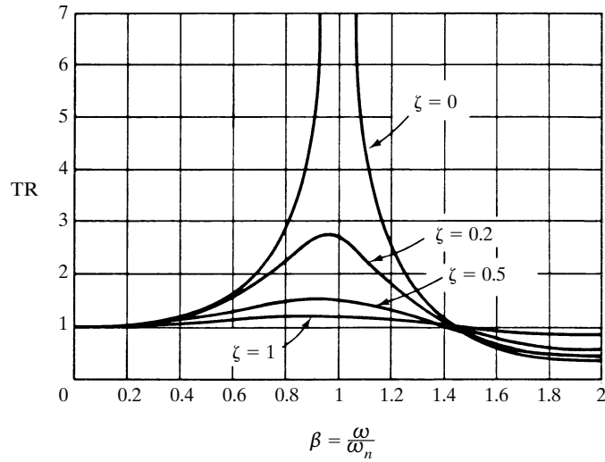
Figure 9-9 Curves of transmissibility \text{TR} versus \beta (= \omega/\omega_n) .
