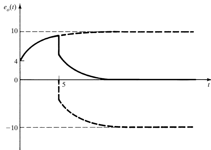
Figure 6-52 Response curve e_o(t) versus t .
