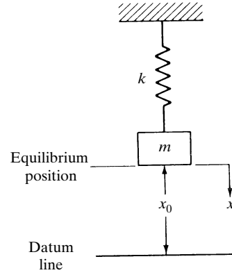
Figure 3–16 Mechanical system.
