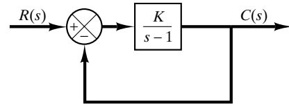
Figure 11-63 Closed-loop system.
