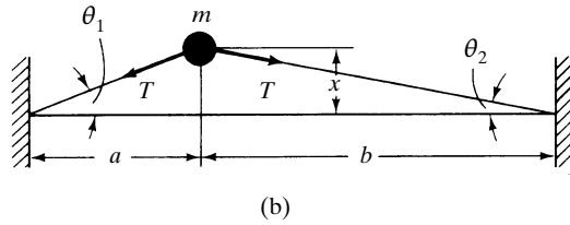
Figure 8-16 (a) Mechanical vibratory system; (b) diagram showing tension forces.
