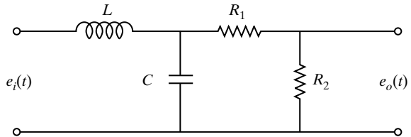
Figure 6-74 Electrical circuit.
