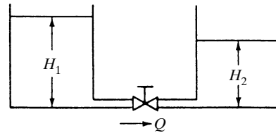
Figure 7-2 Two tanks connected by a short pipe with a valve.
