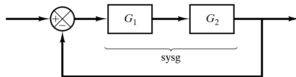
Figure 10-68 Closed-loop system.
