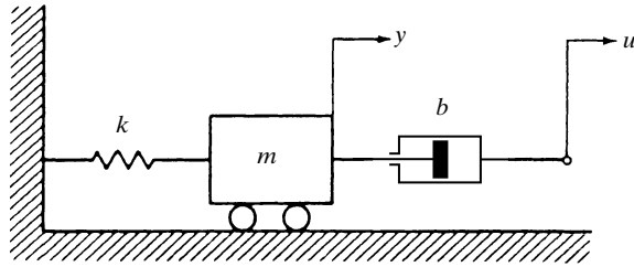
Figure 5-42 Mechanical system.
