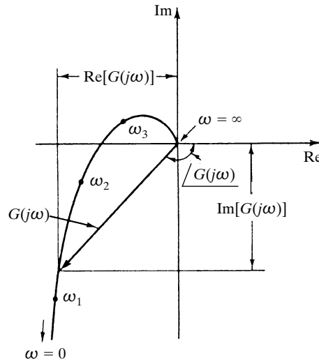
Figure 11-19 Nyquist plot.
