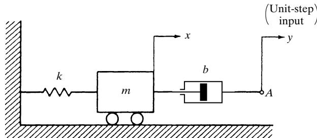
Figure 4-23 Mechanical system.
