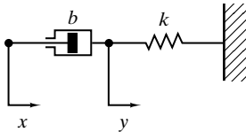
Figure 7-12 Spring-dashpot system.
