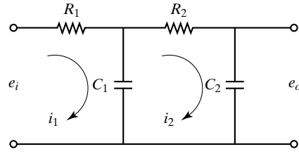
Figure 6-18 Electrical system.
