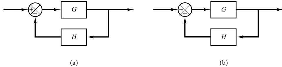
Figure 10–6 (a) Negative feedback system; (b) positive feedback system.
