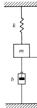
Figure 3-45 Mechanical system.
