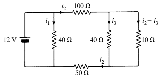
Figure 6-39 Electrical circuit.
