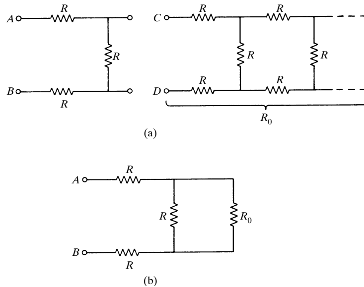
Figure 6-42 Equivalent circuits to the one shown in Figure 6-41.
