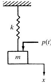
Figure 4-63 Mechanical system.
