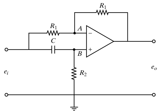
Figure 6-96 Operational-amplifier circuit.
