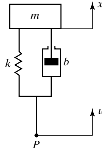
Figure 4-57 Mechanical system.
