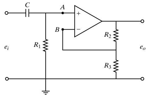
Figure 6-95 Operational-amplifier circuit.
