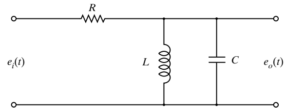
Figure 6-75 Electrical circuit.
