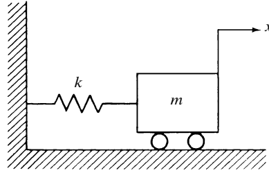
Figure 3-15 Mechanical system.
