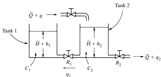
Figure 7-19 Liquid-level system.
