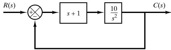
Figure 10-99 Control system.
