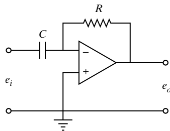
Figure 6-87 Operational-amplifier circuit.
