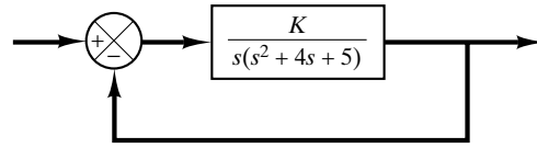
Figure 10–79 Control system.
