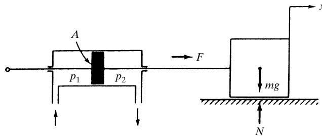
Figure 7-36 Pneumatic system.
