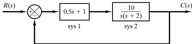
Figure 10-94 Control system.
