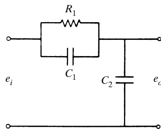
Figure 8-14 Electrical circuit.
