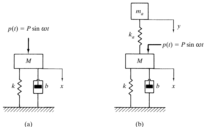
Figure 9-14 (a) Machine supported by a spring and damper; (b) machine with a dynamic vibration absorber.
