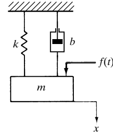
Figure 4-1 Mechanical system.
