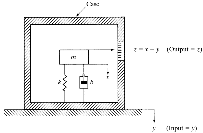
Figure 9-30 Translational accelerometer.
