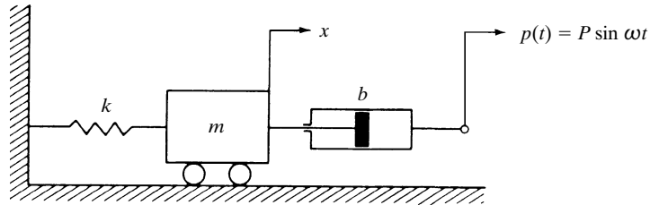
Figure 9-24 Mechanical system.
