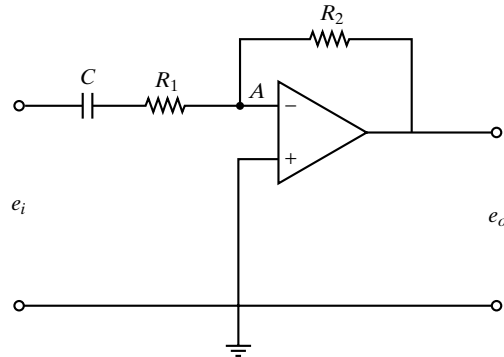
Figure 6-94 Operational-amplifier circuit.
