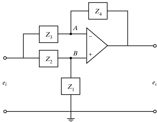
Figure 6-66 Operational-amplifier circuit.
