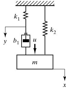
Figure 4-25 Mechanical system.
