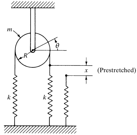
Figure 3-26 Spring-pulley system.
