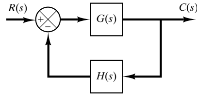
Figure 10–40 Control system.
