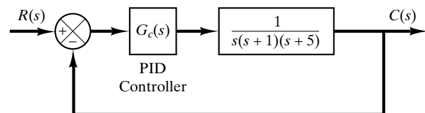
Figure 10–58 PID-controlled system.
