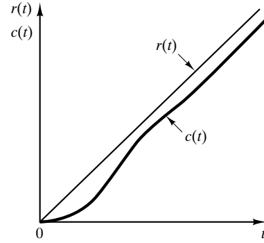
Figure 10-37 Response of a type 1 unity-feedback system to a ramp input.
