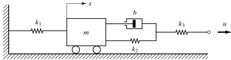
Figure 4-54 Mechanical system.
