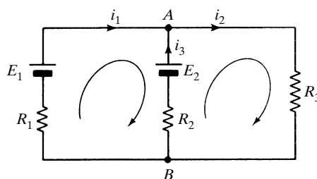
Figure 6-9 Electrical circuit.
