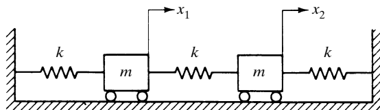
Figure 9-17 Mechanical system with two degrees of freedom.
