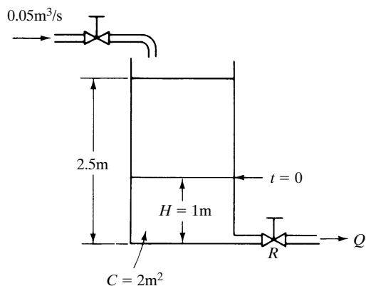
Figure 7-29 Liquid-level system.
