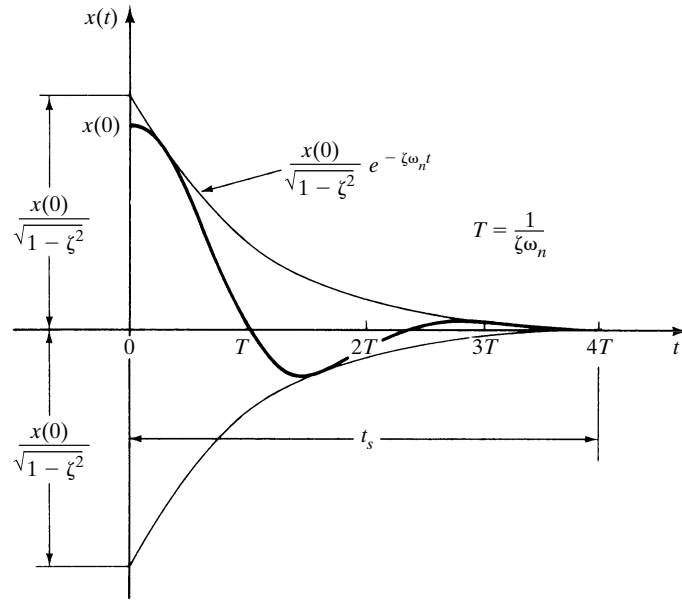
Figure 8-9 Typical response curve of the system shown in Figure 8-6 and its envelope exponentials.
