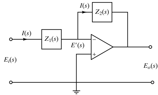
Figure 6-63 Operational-amplifier circuit.
