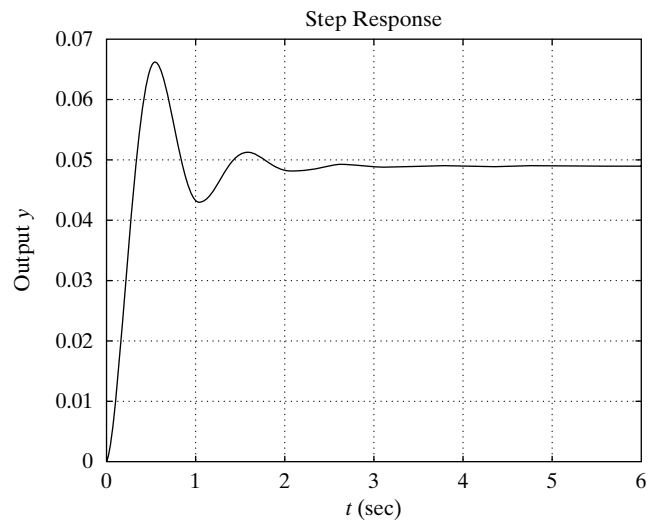
Figure 5-30 Step-response curve.
