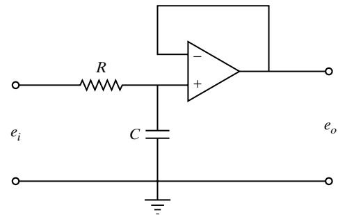
Figure 6-90 Operational-amplifier circuit.
