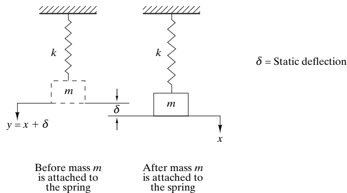
Figure 3-10 Spring-mass system.
