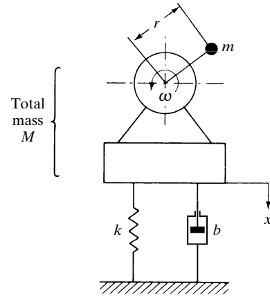
Figure 9-6 Unbalanced machine resting on shock mounts.
