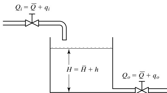
Figure 7-8 Liquid-level system.
