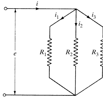
Figure 6-3 Parallel circuit.
