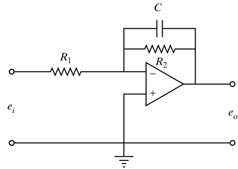
Figure 6-89 Operational-amplifier circuit.
