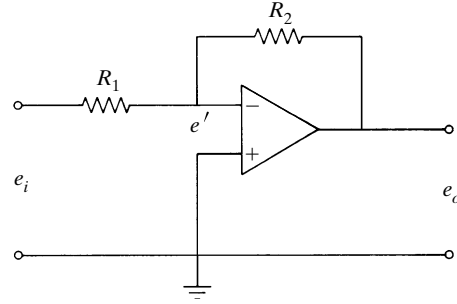
Figure 6-32 Operational-amplifier system.
