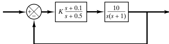
Figure 11–70 Control system.
