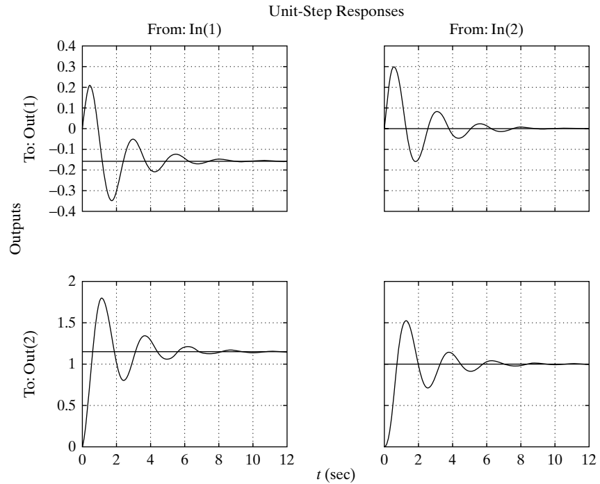
Figure 5-4 Unit-step response curves.
