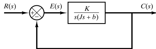
Figure 10-75 Closed-loop system.
