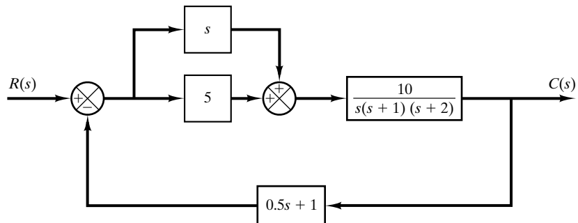
Figure 10-95 Control system.
