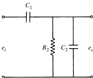
Figure 6-50 Electrical circuit.
