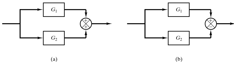
Figure 10-5 Parallel-connected systems. (a) G_1 + G_2 ; (b) G_1 - G_2 .
