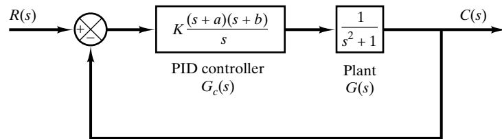
Figure 10–108 PID-controlled system.
