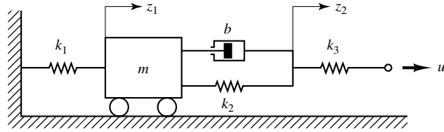
Figure 5-47 Mechanical system.
