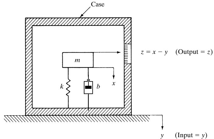
Figure 9-29 Seismograph.
