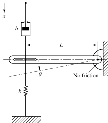
Figure 4-56 Mechanical system.
