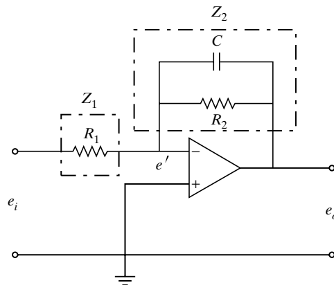
Figure 6-64 Operational-amplifier circuit.
