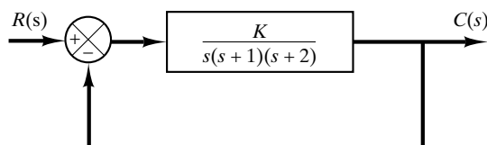
Figure 10–41 Control system.
