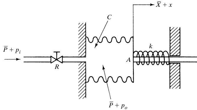
Figure 7-33 Pneumatic system.
