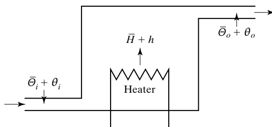
Figure 7-14 Air-heating system.
