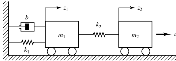
Figure 5-48 Mechanical system.
