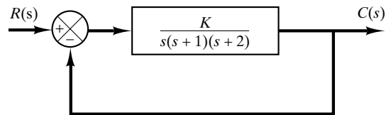
Figure 10–39 Control system.
