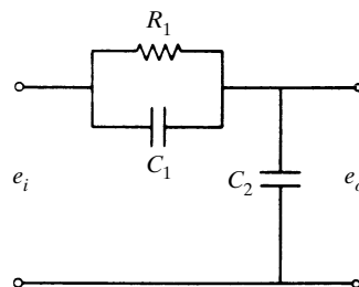
Figure 6-51 Electrical circuit.
