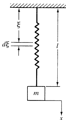
Figure 3-34 Spring-mass system.
