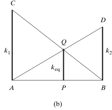
Figure 3-22 (a) System consisting of two springs in series; (b) diagram showing the equivalent spring constant.
