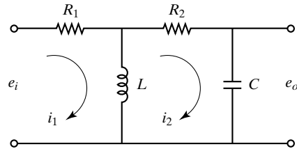
Figure 6-76 Electrical circuit.
