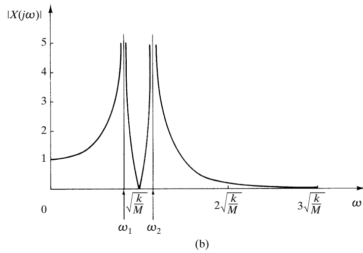
Figure 9-15 (a) Curve of amplitude versus frequency for the system of Figure 9-14(a); (b) curve of amplitude versus frequency for the system of Figure 9-14(b).
