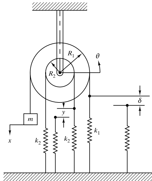
Figure 3–46 Mechanical system.
