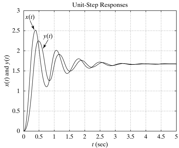
Figure 4-12 Step-response curves x(t) and y(t) .
