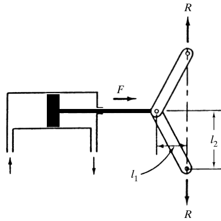
Figure 7-35 Toggle joint.
