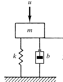
Figure 5-2 Mechanical system.
