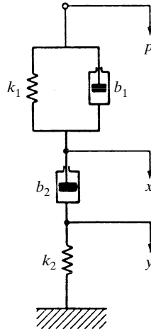
Figure 11-54 Mechanical system.
