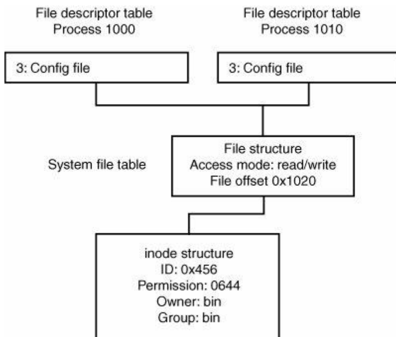
Figure 10-1. File data structures after fork
