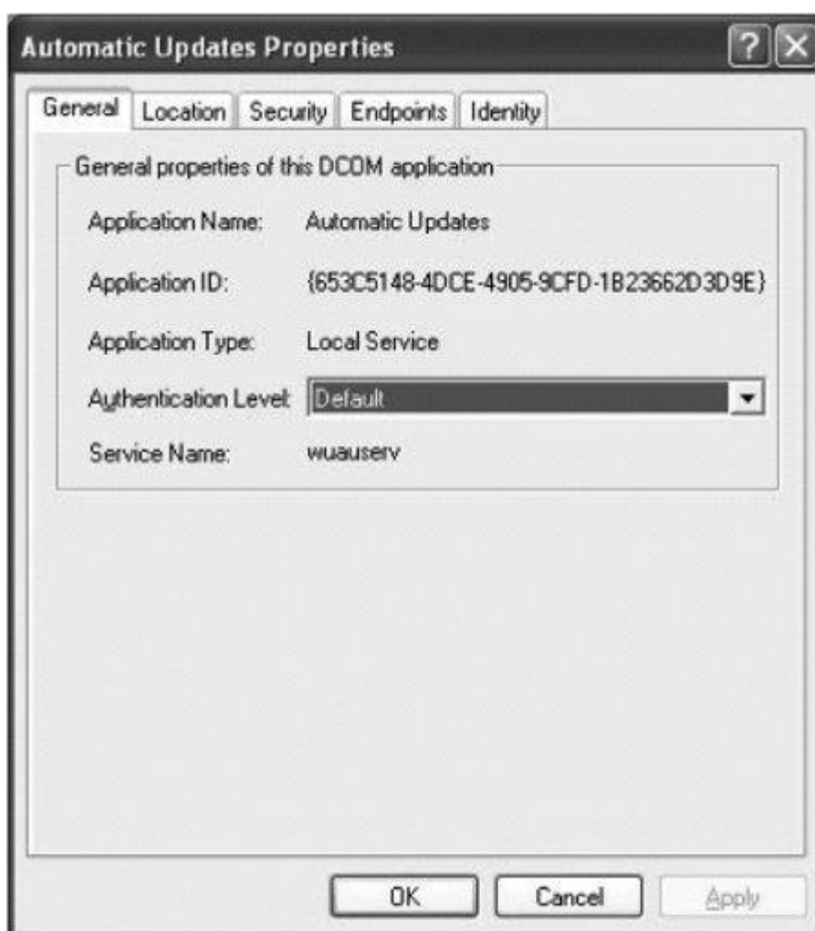
Figure 12-4. Viewing properties of COM objects
