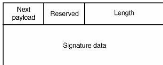
Figure 16-10. ISAKMP signature payload header
