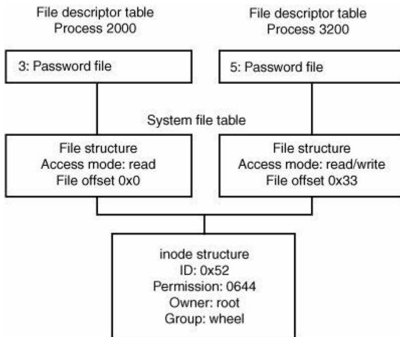
Figure 10-2. Independent opens of the same file
