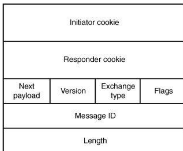
Figure 16-1. ISAKMP protocol header
