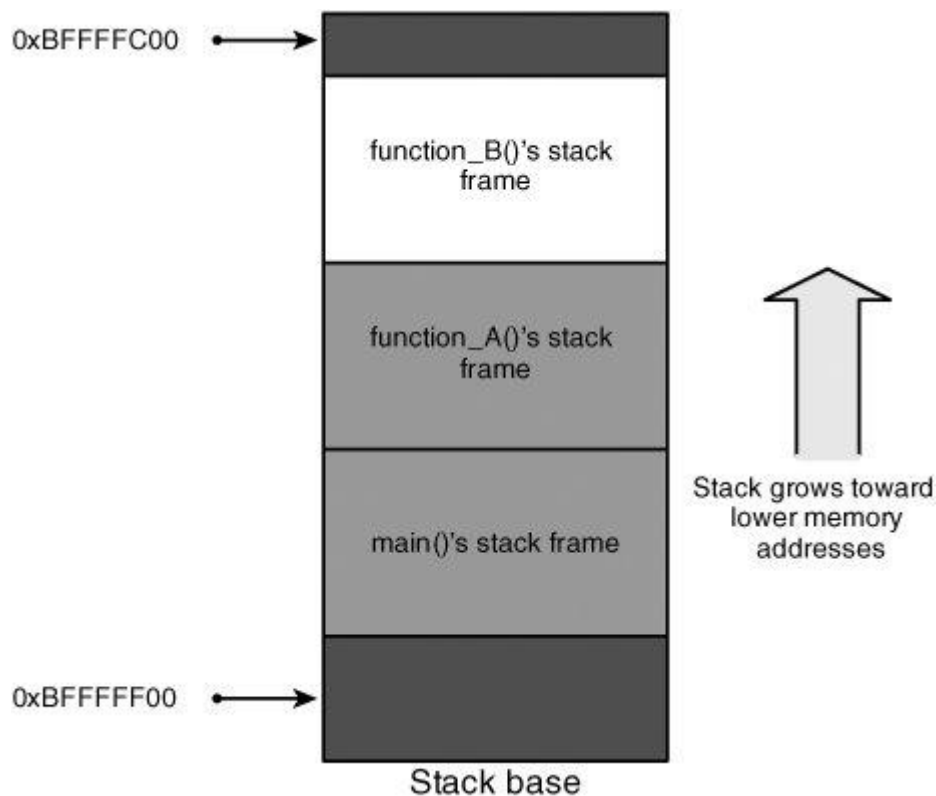
Figure 5-2. Stack while in function_B()
