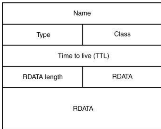
Figure 16-21. DNS resource record data structure
