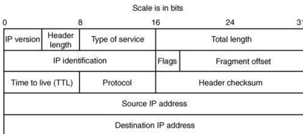
Figure 14-1. IPv4 header diagram
