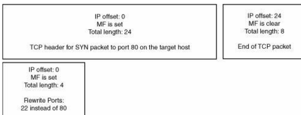
Figure 15-7. TCP ports rewrite fragment attack
