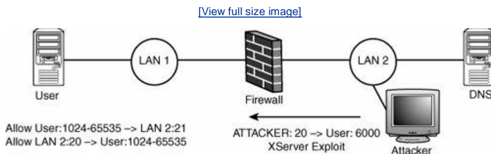
Figure 15-4. TCP source port 20 attack for stateless firewalls
