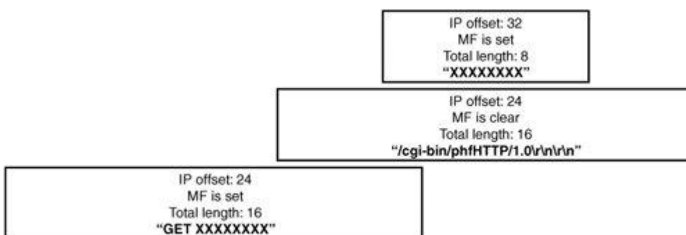
Figure 14-8. Windows overlap semantics
