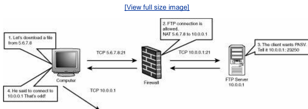
Figure 15-9. Active FTP failure caused by NAT
