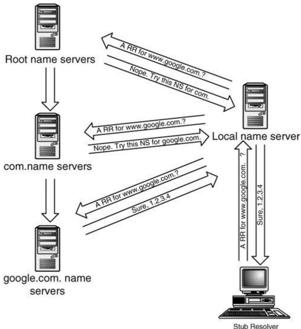
Figure 16-17. DNS request traffic
