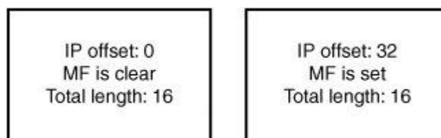
Figure 14-4. Malicious IP fragments
