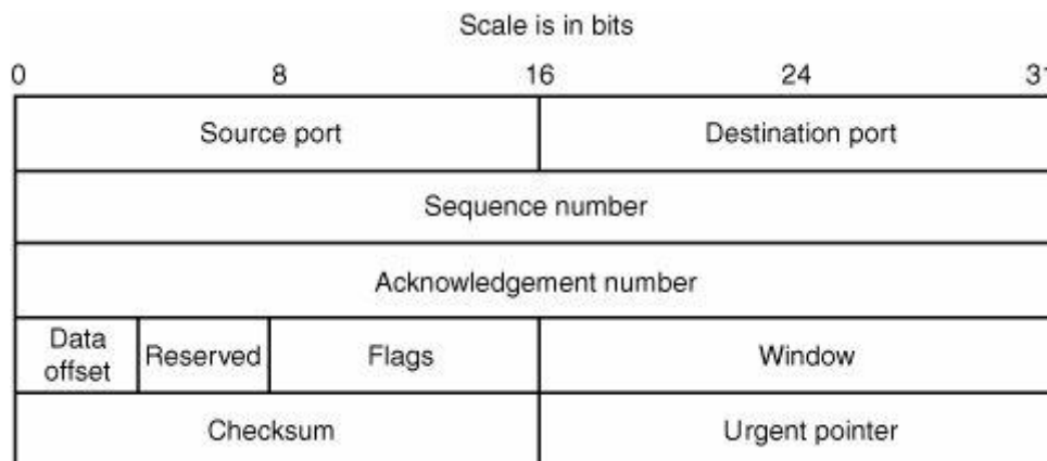
Figure 14-10. TCP header
