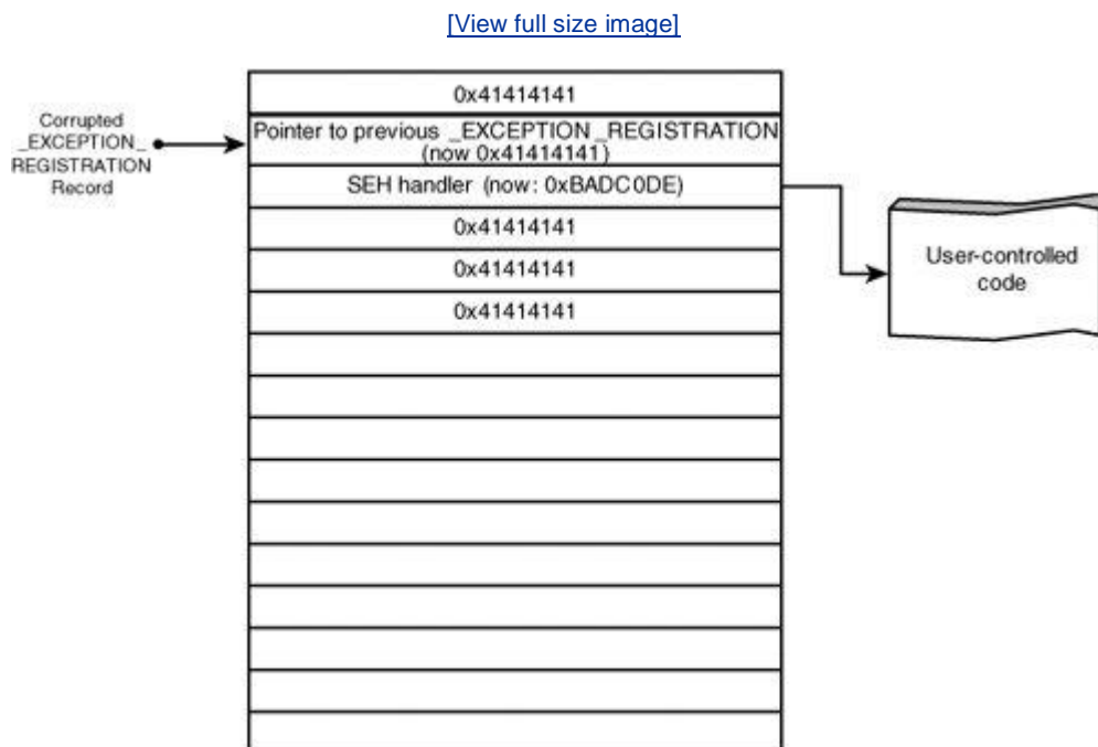
Figure 5-8. SEH exploit
