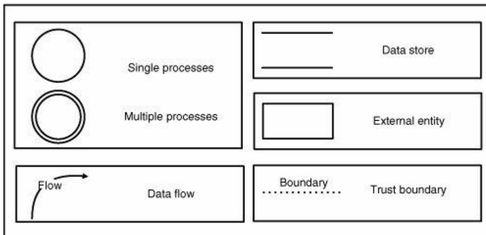
Figure 2-2. DFD elements
