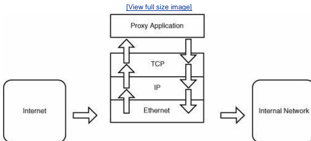
Figure 15-2. Proxy firewall data flow
