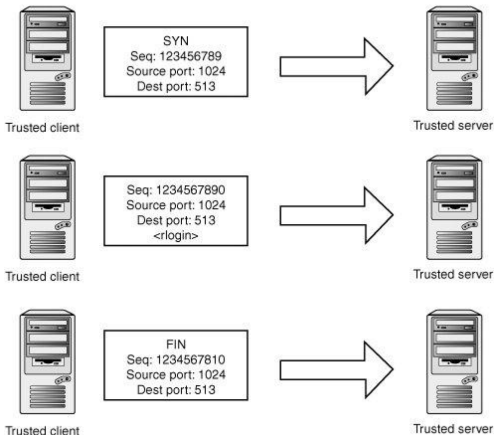
Figure 14-22. Blind spoofing attack
