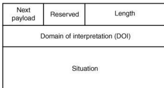
Figure 16-3. ISAKMP security association payload header
