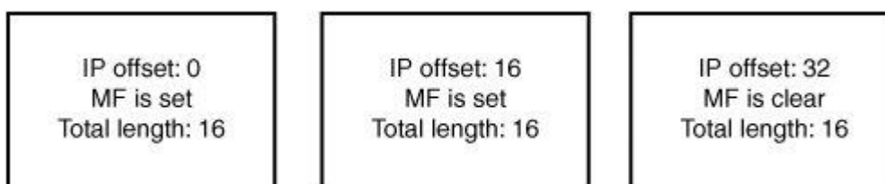
Figure 14-3. IP fragmentation reassembly
