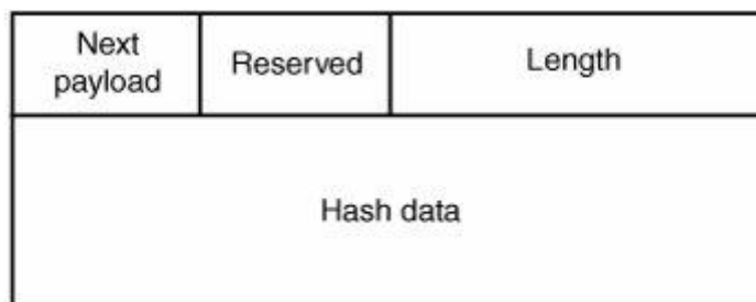
Figure 16-9. ISAKMP hash payload header
