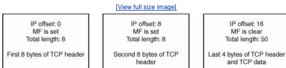
Figure 15-5. Straightforward fragment attack
