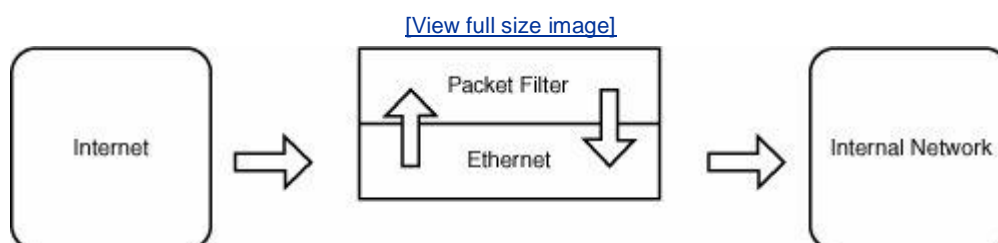
Figure 15-1. Packet-filtering data flow
