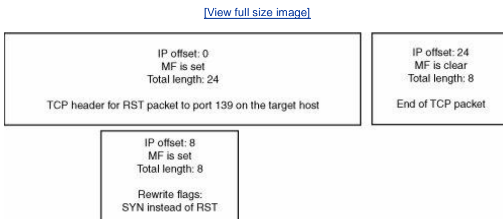
Figure 15-6. TCP flags rewrite fragment attack
