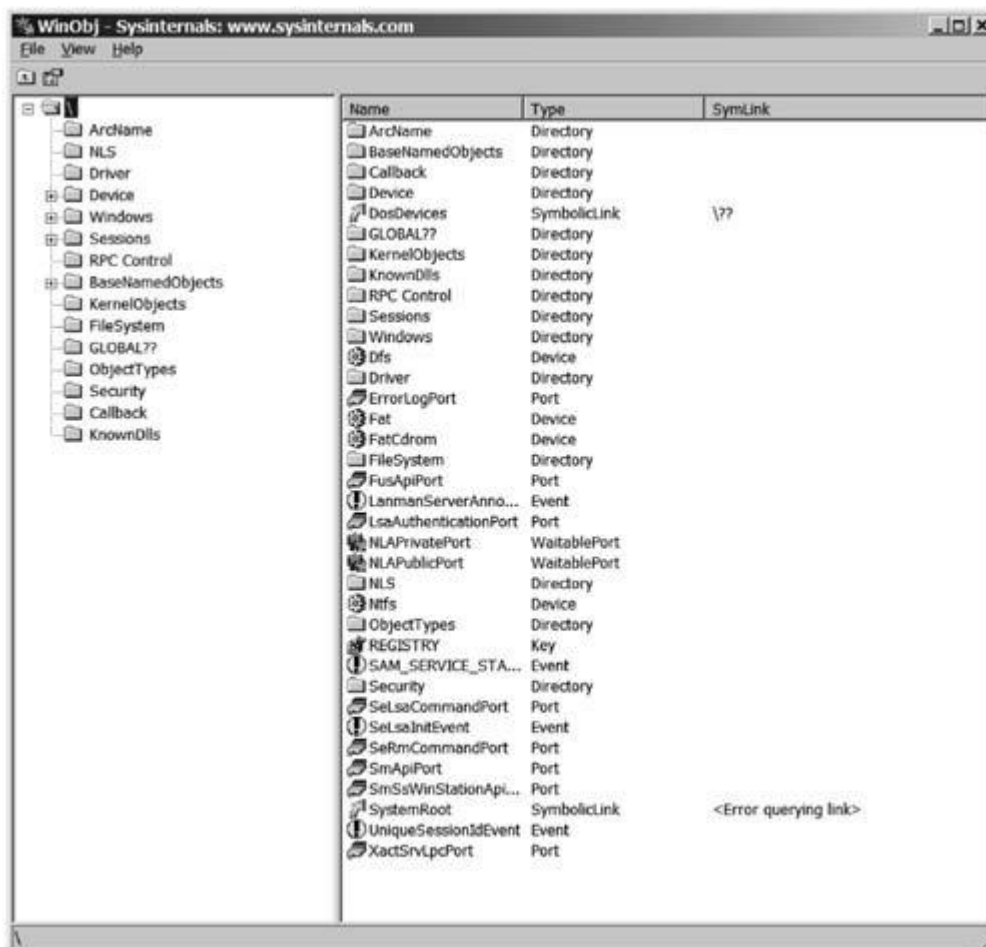
Figure 11-1. The WinObj main window
