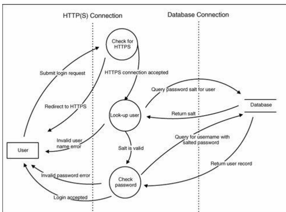
Figure 2-6. A DFD showing a login vulnerability
