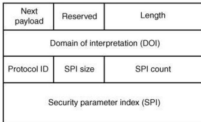
Figure 16-13. ISAKMP delete payload header
