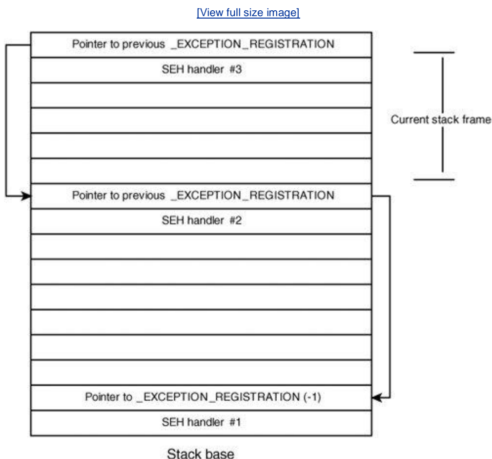
Figure 5-7. Windows SEH layout
