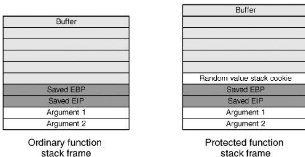
Figure 5-13. Stack frame with and without cookies
