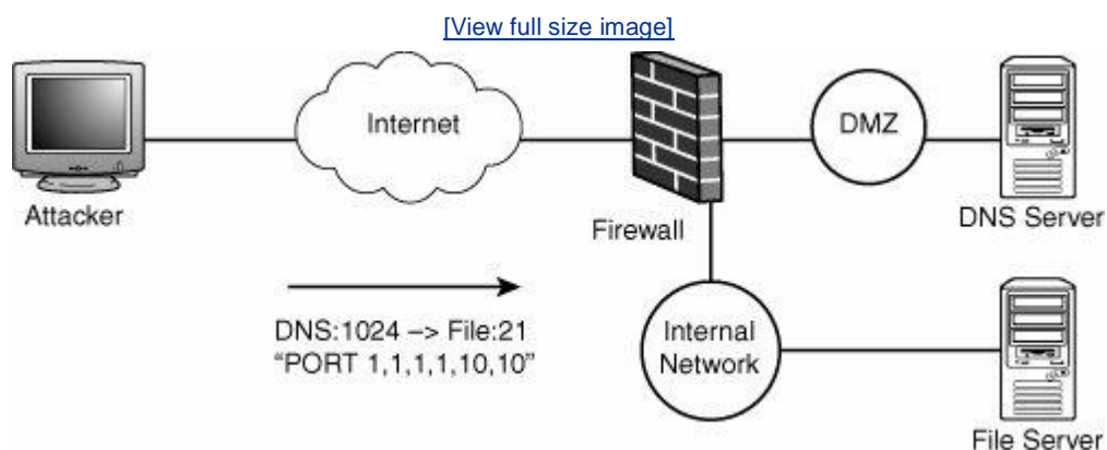
Figure 15-14. Spoofing for state table manipulation
