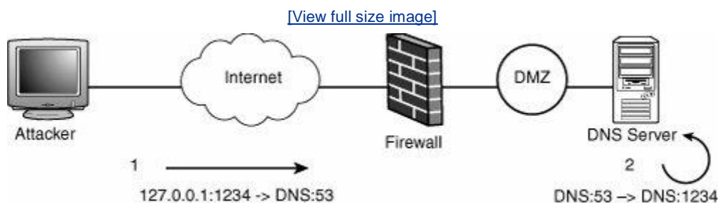
Figure 15-13. Spoofing to elicit a response
