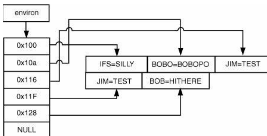
Figure 10-4. Process environment immediately after an execve()
