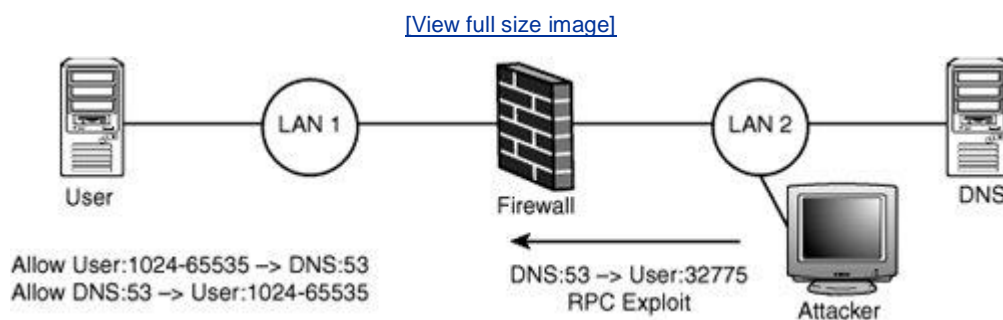
Figure 15-3. UDP source port 53 attack for stateless firewalls
