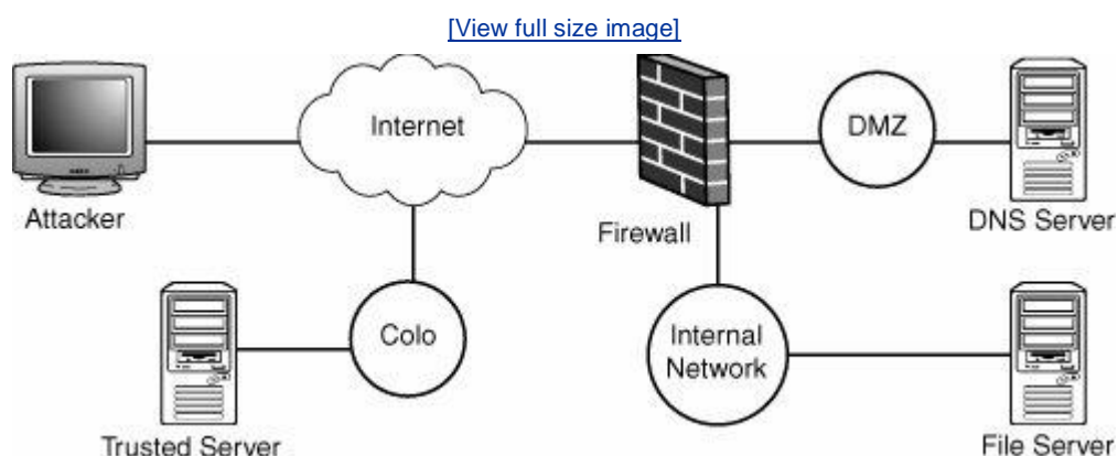
Figure 15-11. Spoofing from an external trusted source
