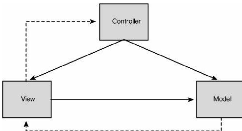
Figure 17-4. Mode- View-Controller (MVC) architecture
