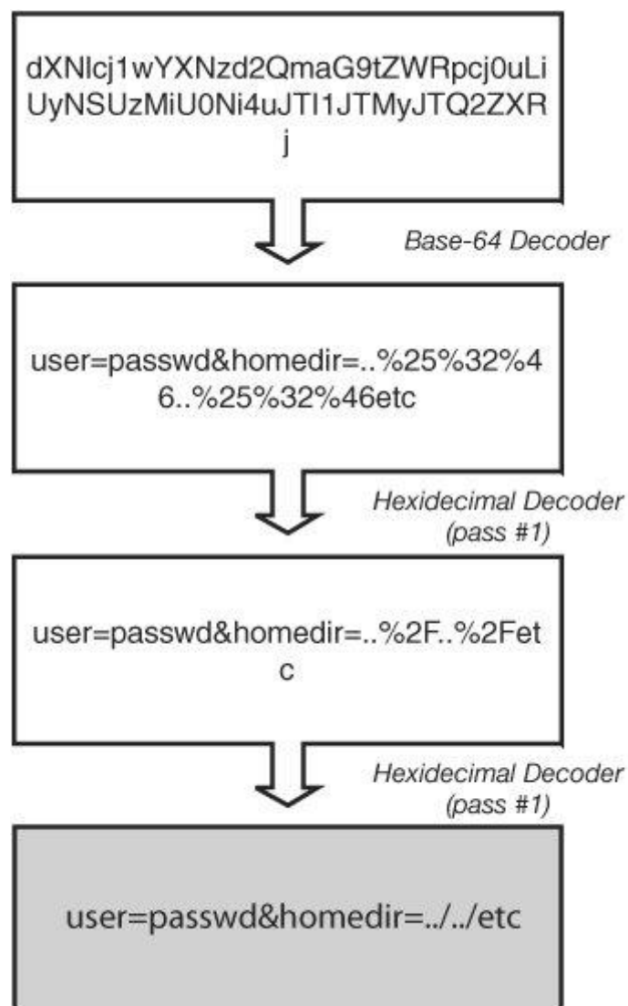
Figure 8-3. Encoded Web data
