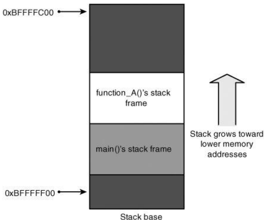
Figure 5-1. Stack while in function_A()
