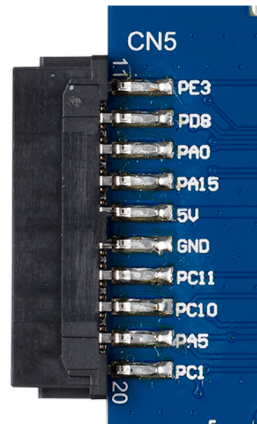
Figure 17. Bottom silkscreen STMod+ connector
