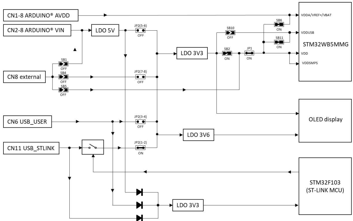
Figure 8. STM32WB5MM-DK power tree
