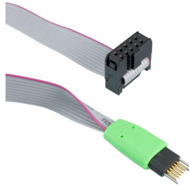
Figure 19. TC2050-IDC-NL cable
