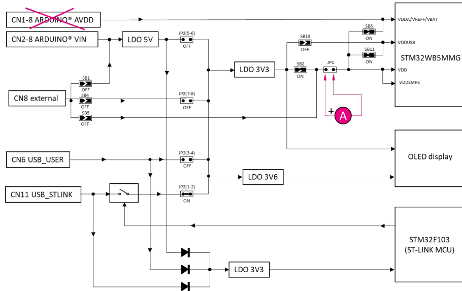
Figure 9. Current measurement with an ammeter
