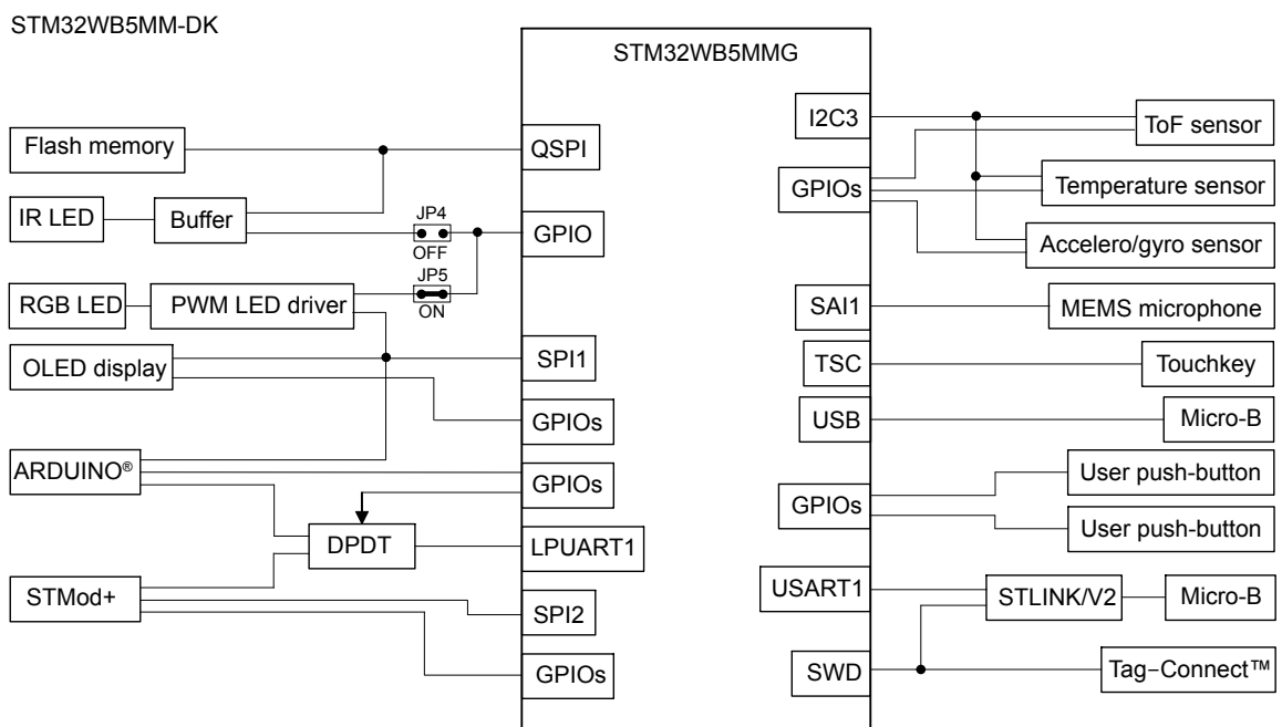
Figure 3. STM32WB5MM-DK hardware block diagram
