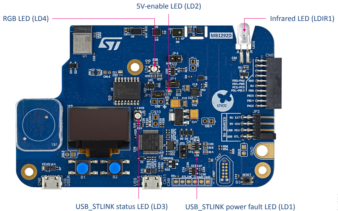
Figure 11. LEDs location
