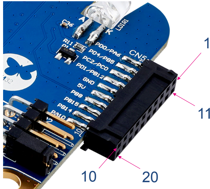
Figure 15. STMod+ connector (CN5)
